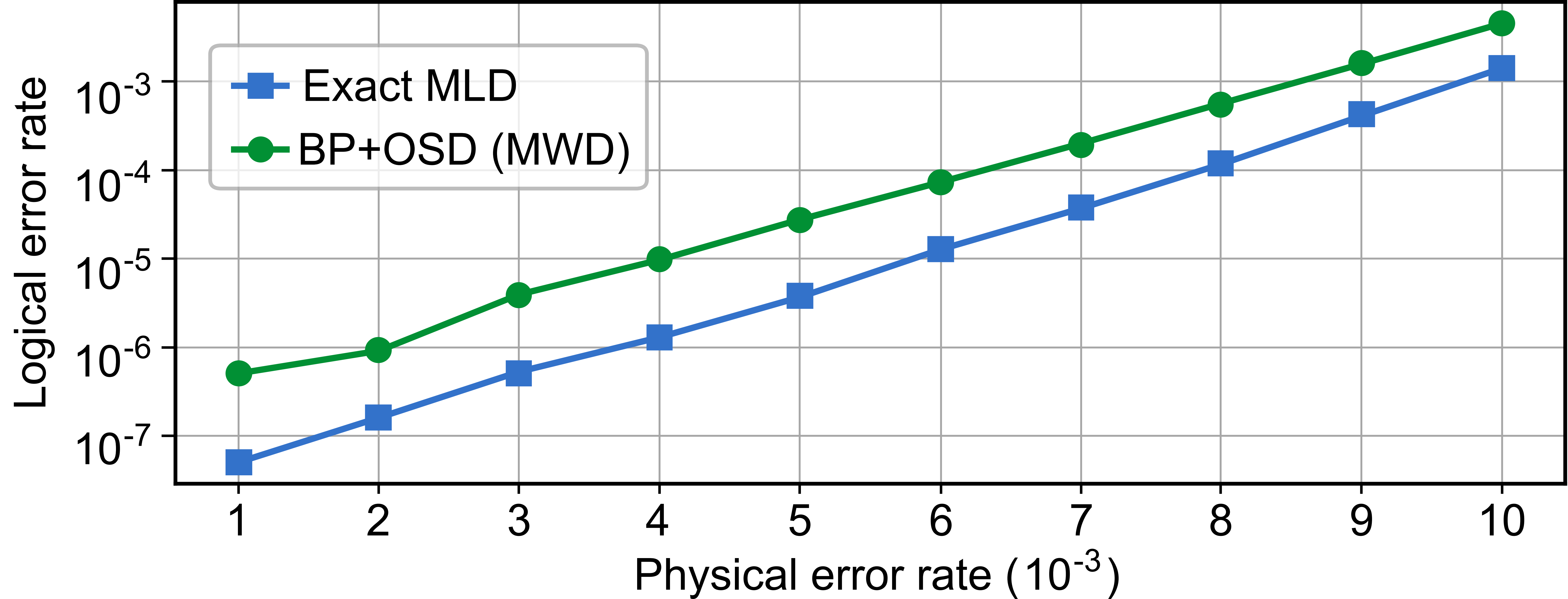
(a) Goal 1: bridge the LER gap between the MLD and MWD
