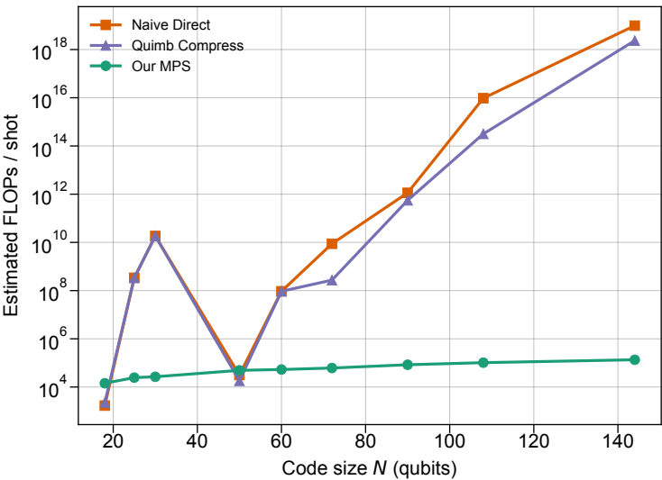
FLOPs Scaling vs Code Size
