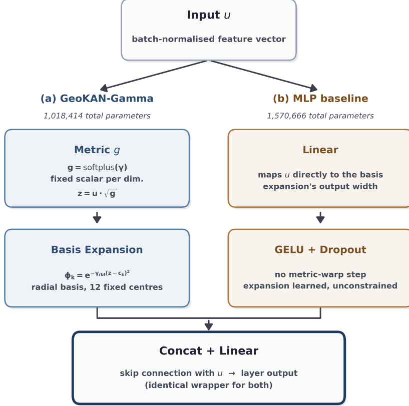
Fig. 4 Controlled architecture ablation: the GeoKAN layer (Section 4.5) replaced by a matched-budget conventional learned layer, with the rest of the architecture (Section 4.6) unchanged.
