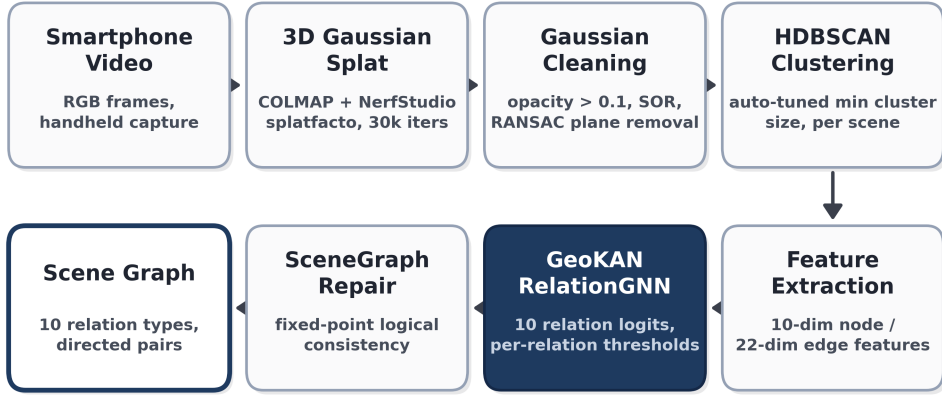
Fig. 1 The LogicSplat pipeline, from smartphone video to scene graph.
