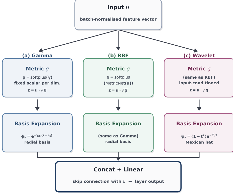
Fig. 2 Internal computation of a single GeoKAN layer, showing where the three variants differ: the metric computation g , and the basis function applied after warping.
