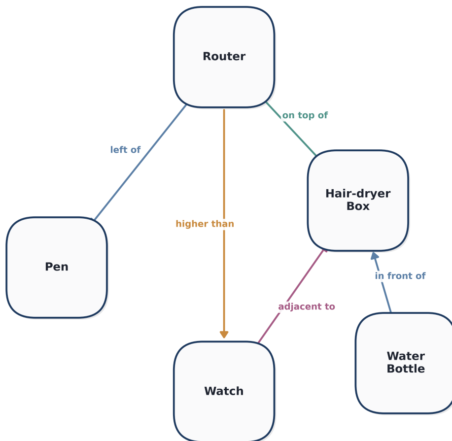
Predicted scene graph (post-repair), scene_06 one verified-correct example of each relation type that occurs in this scene
