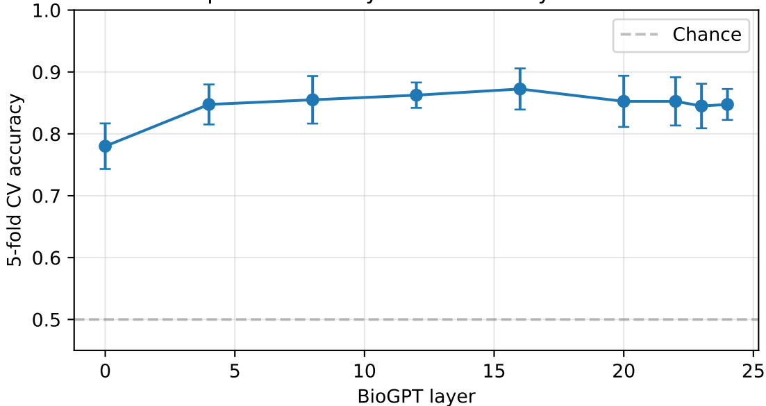
Linear probe accuracy for uncertainty classification
