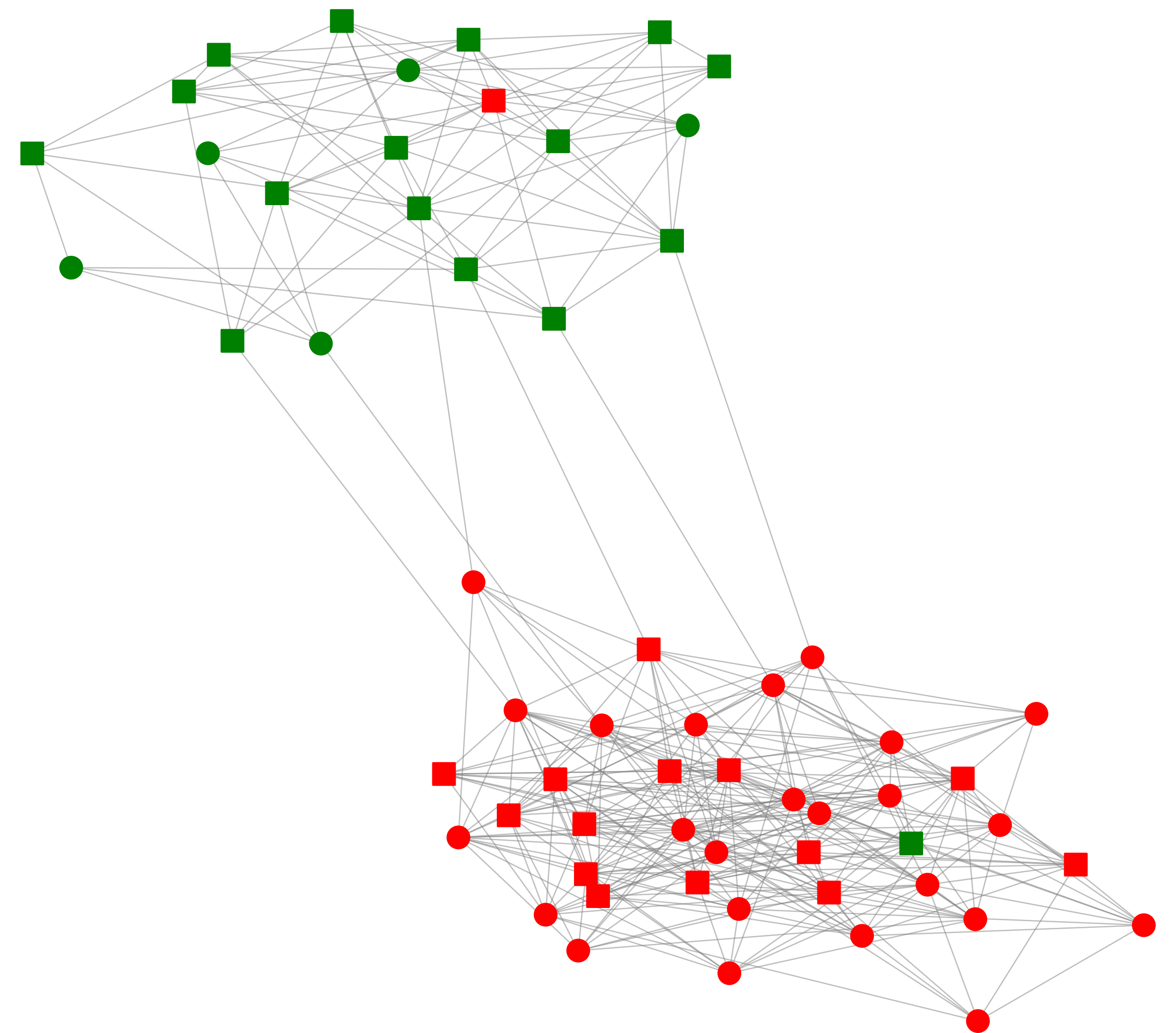
Original Graph
