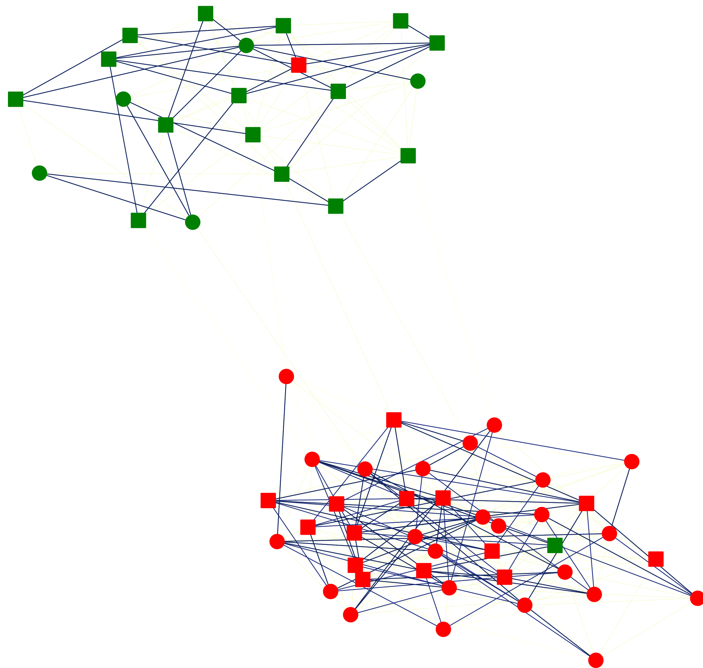
Learned Graph
