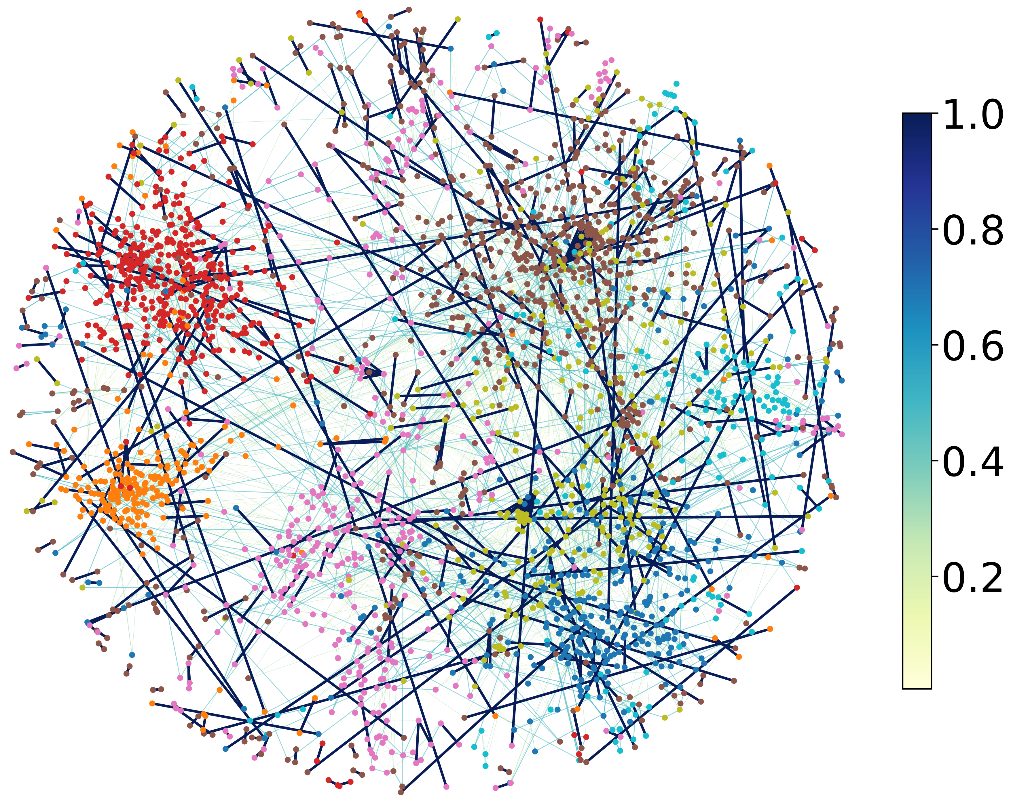
GAT Attention
