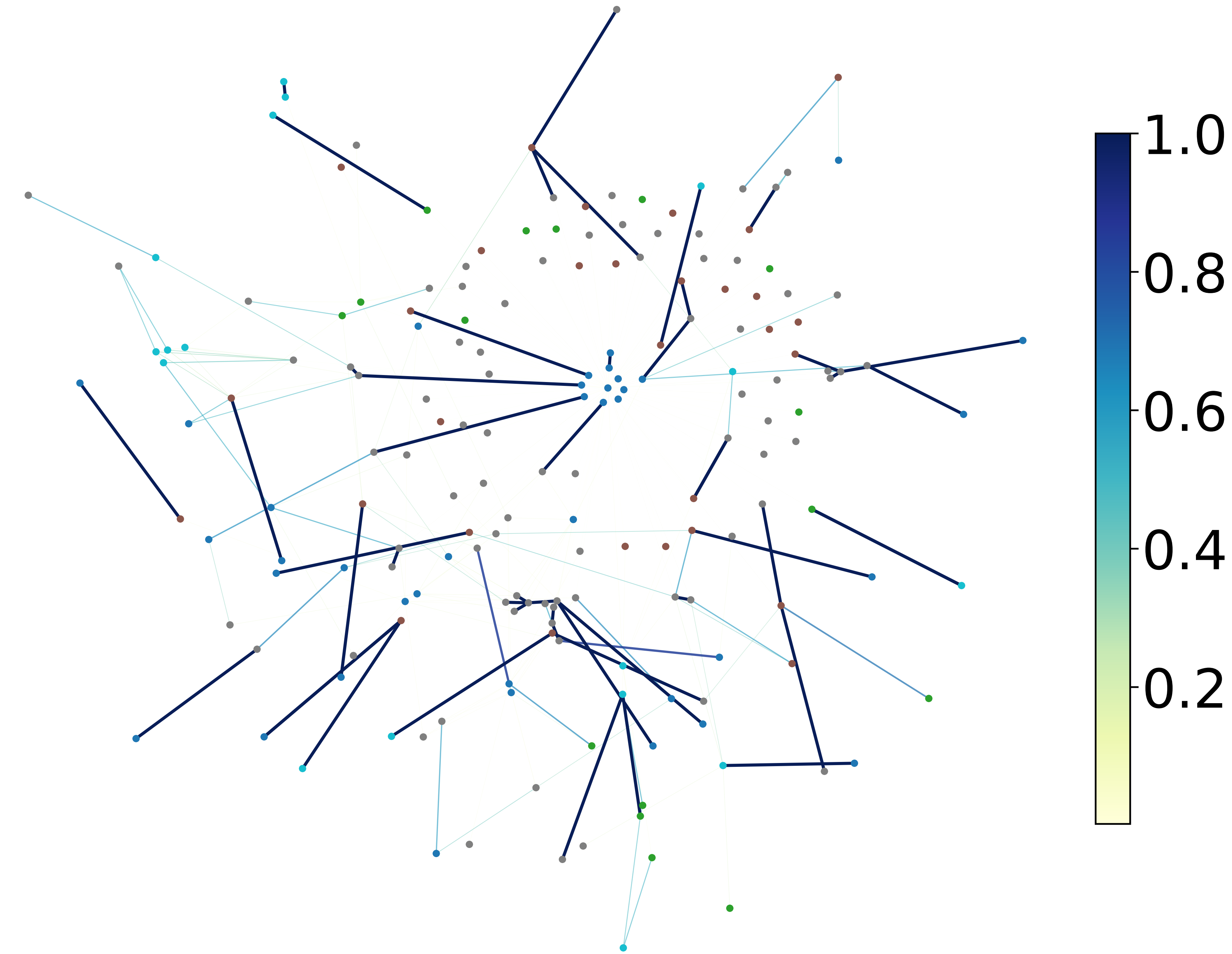
GAT Attention
