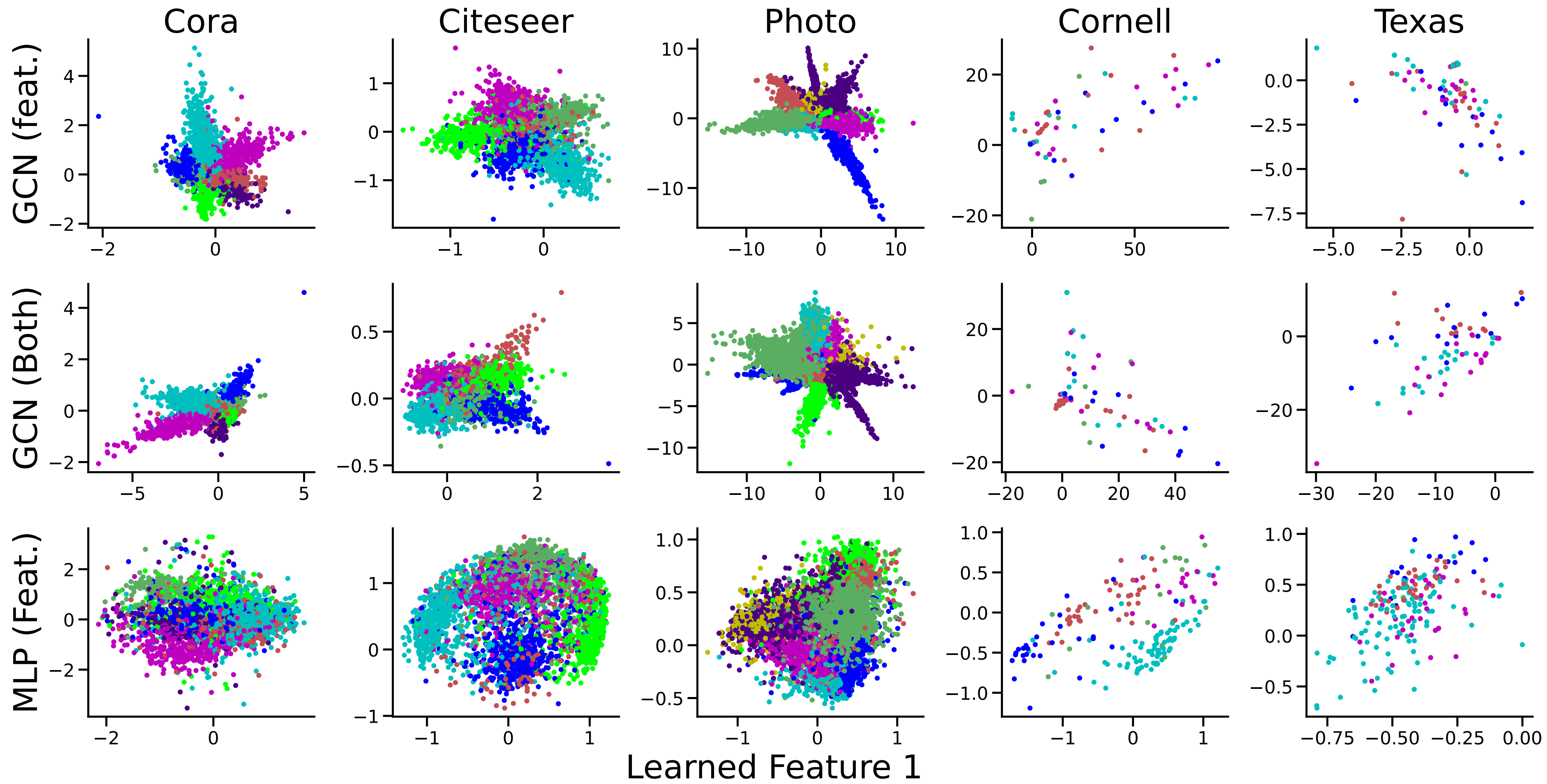
Learned Feature 2
