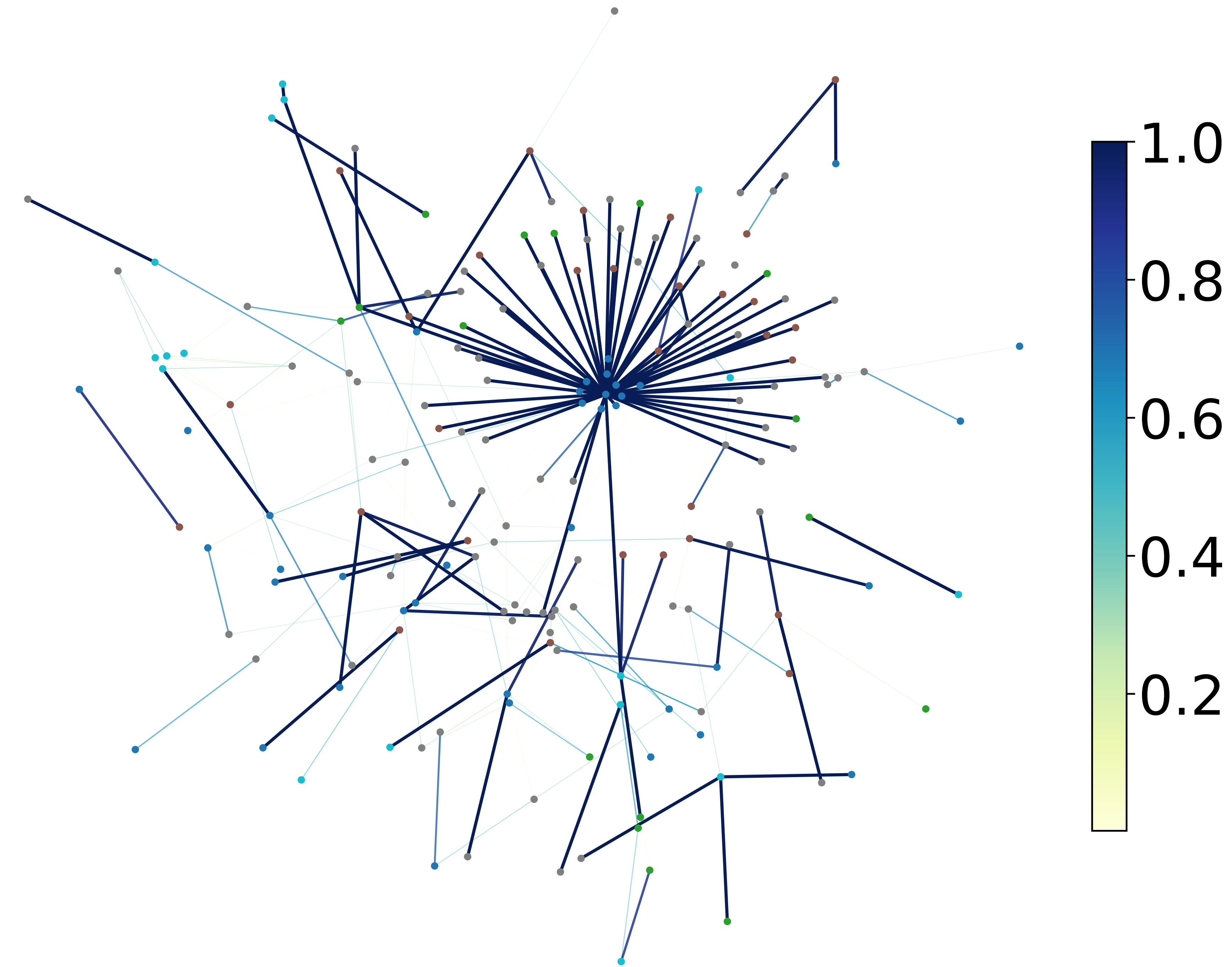
GAT Attention
