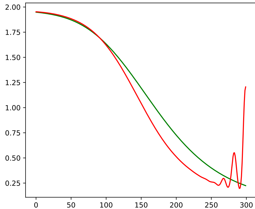
train loss
