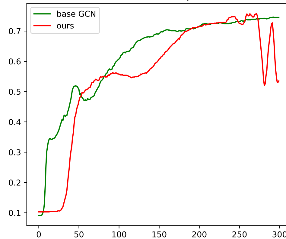
Test Accuracy
