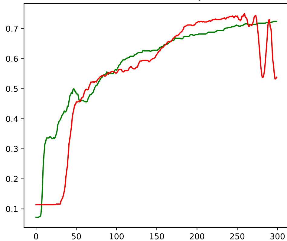
Validation accuracy
