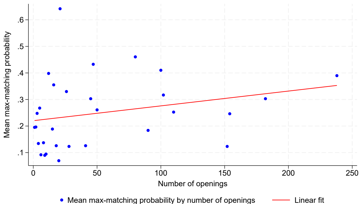
Figure 2: Relationship between max-matching probability and number of openings
