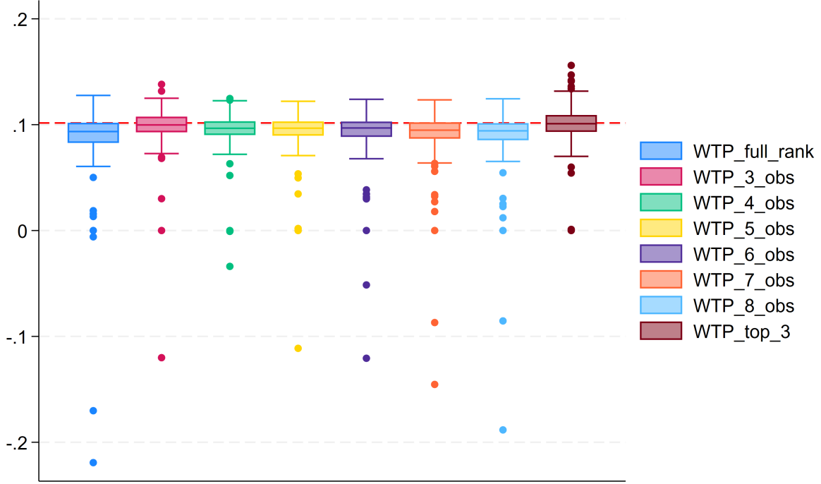
Figure 6: Distribution of the simulated 1 - \exp(-\hat{\beta}^x/\hat{\beta}^w) , B = 300
