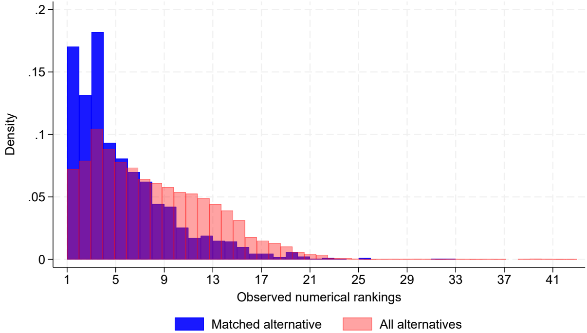
Figure 1: Distribution of rankings
