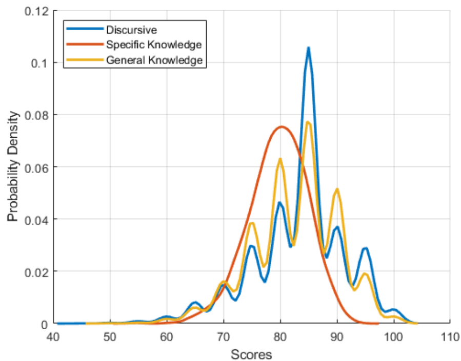
Figure 4: Distribution of exam components' scores
