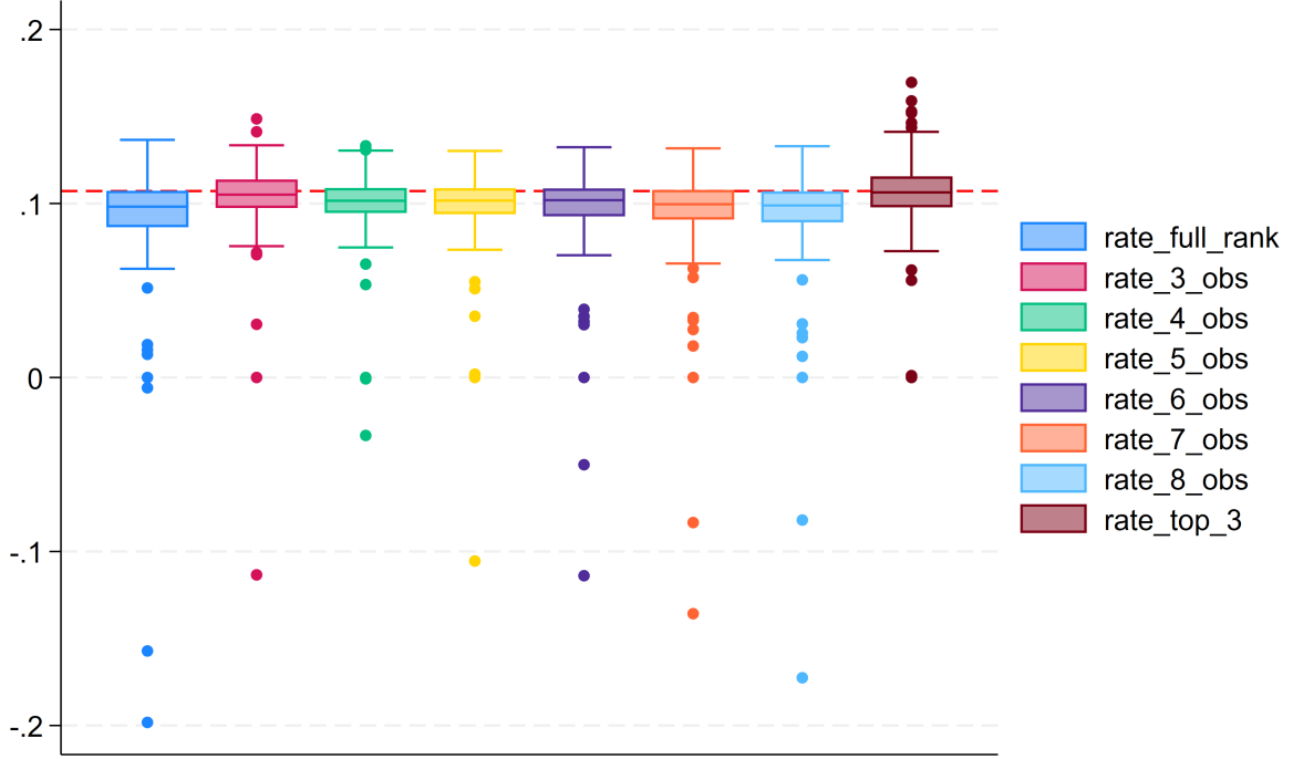
Figure 5: Distribution of the simulated \hat{\beta}^x/\hat{\beta}^w , B = 300
