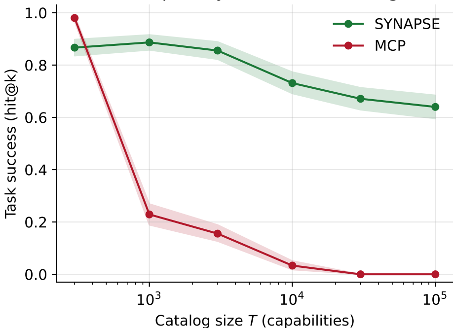
Correct-capability retrieval vs catalog size
