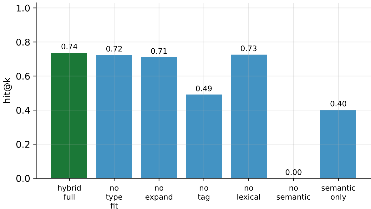
Resolver ablation: contribution of each component
