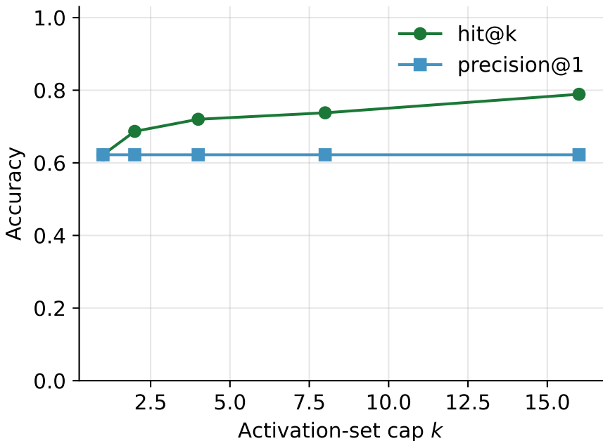
Accuracy vs activation-set size k
