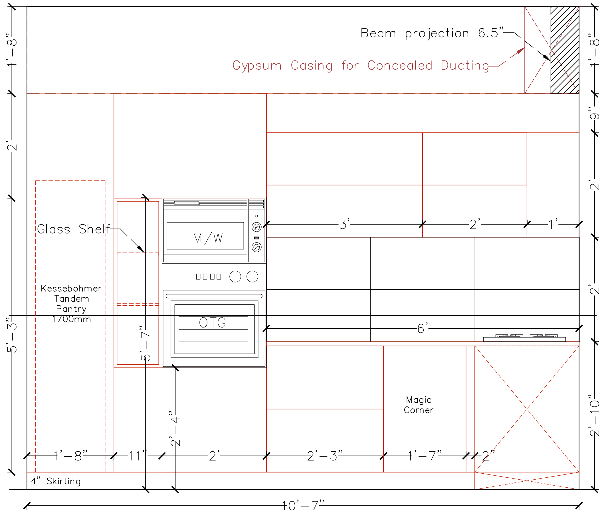
Kitchen — Elevation D
