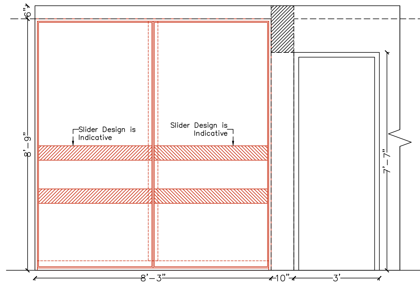
MBR - Sliding Wardrobe - Elevation
