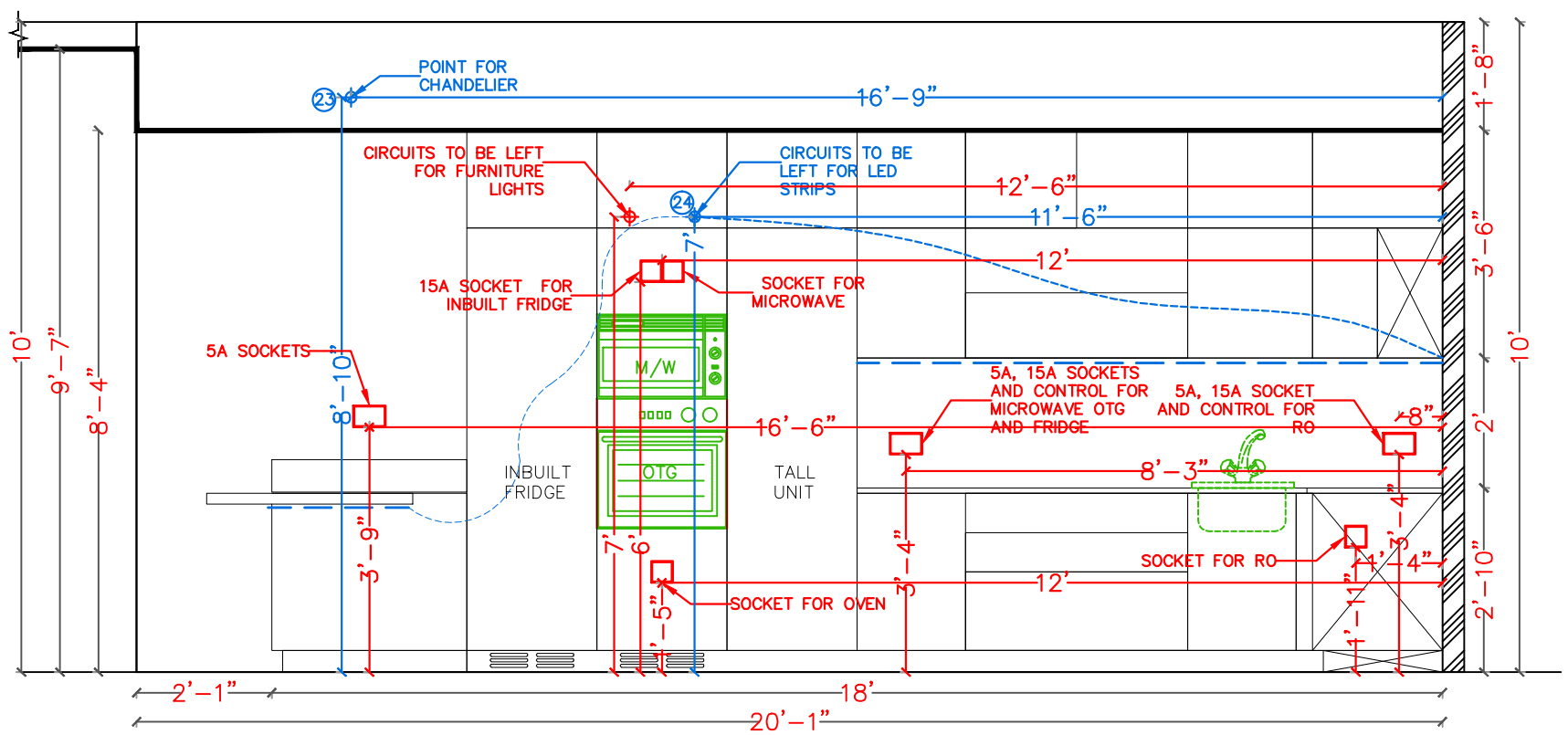
KITCHEN - SERVICE COUNTER
