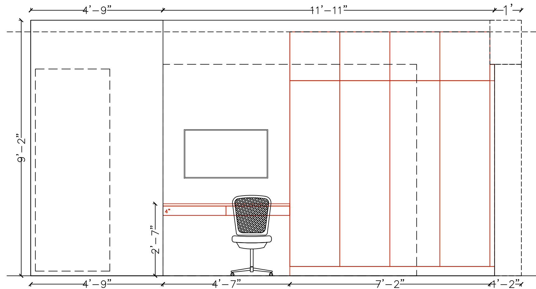
Parents Bedroom – Wardrobe & TV Elevation
