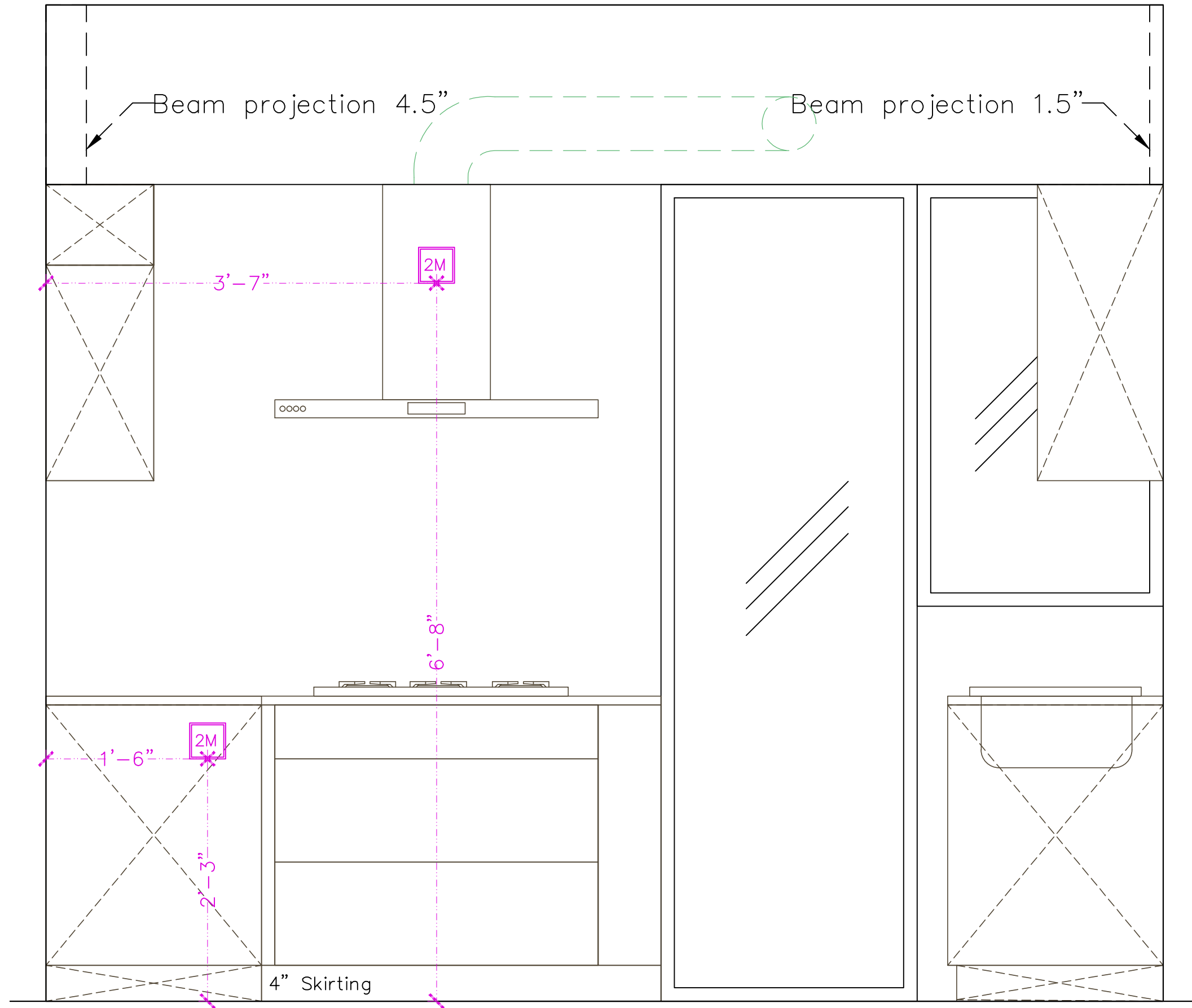
Kitchen — Elevation A
