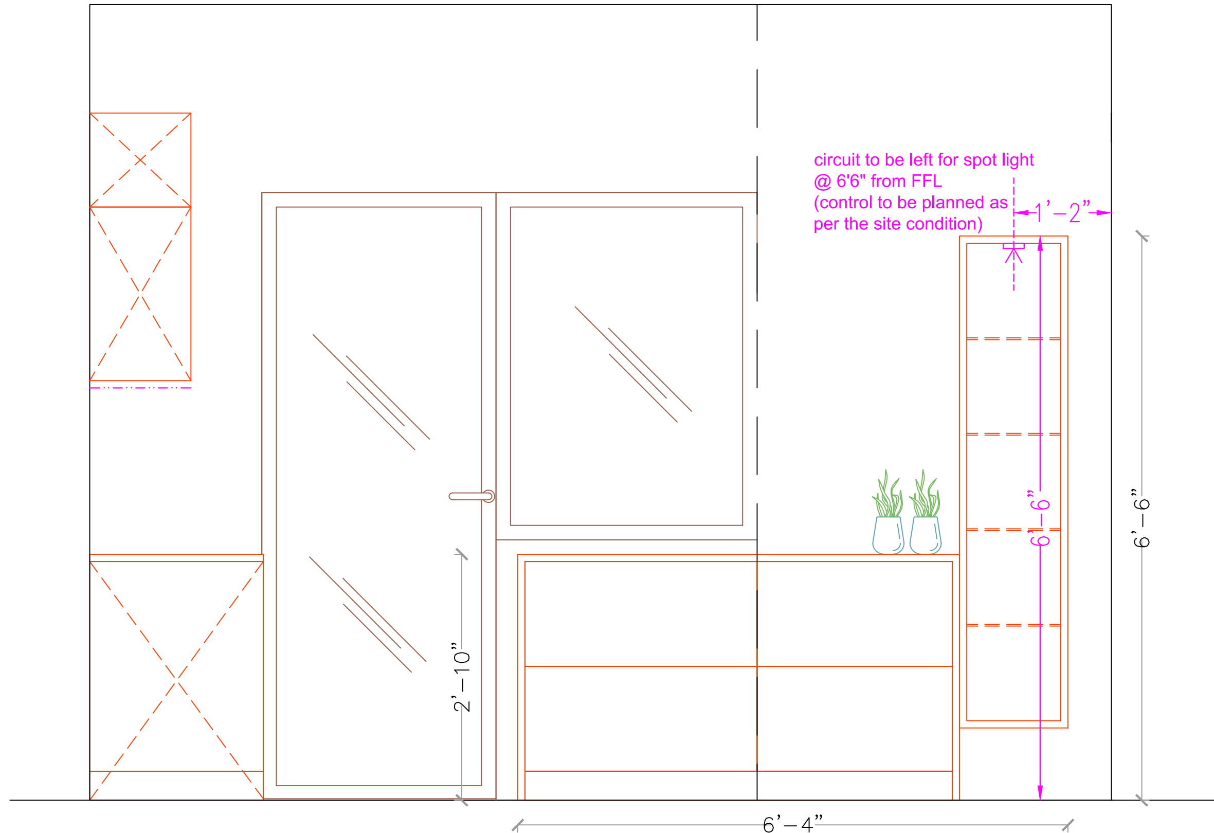
SERVICE COUNTER SIDE ELEVATION
