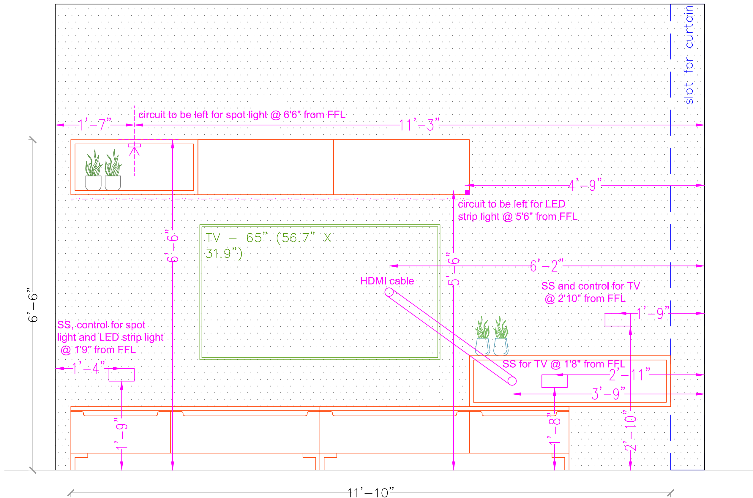
LIVING AREA - TV UNIT - ELEVATION
