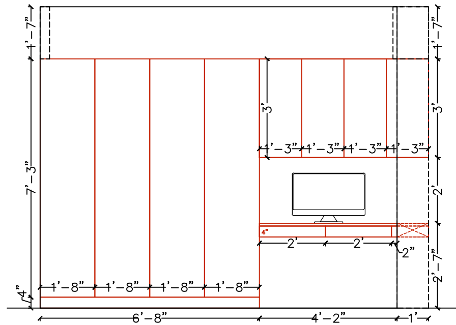
Guest Bedroom – Wardrobe & Study Elevation
