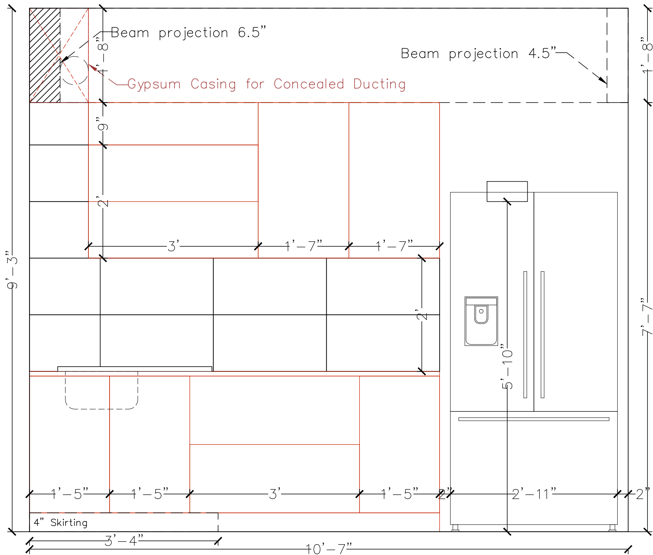
Kitchen — Elevation B
