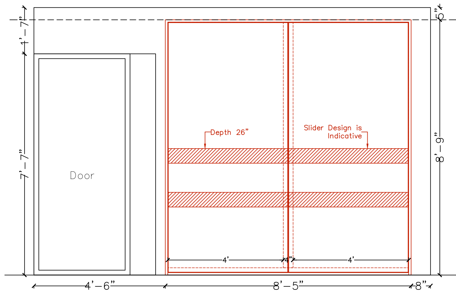
Kids – Sliding Wardrobe – Elevation
