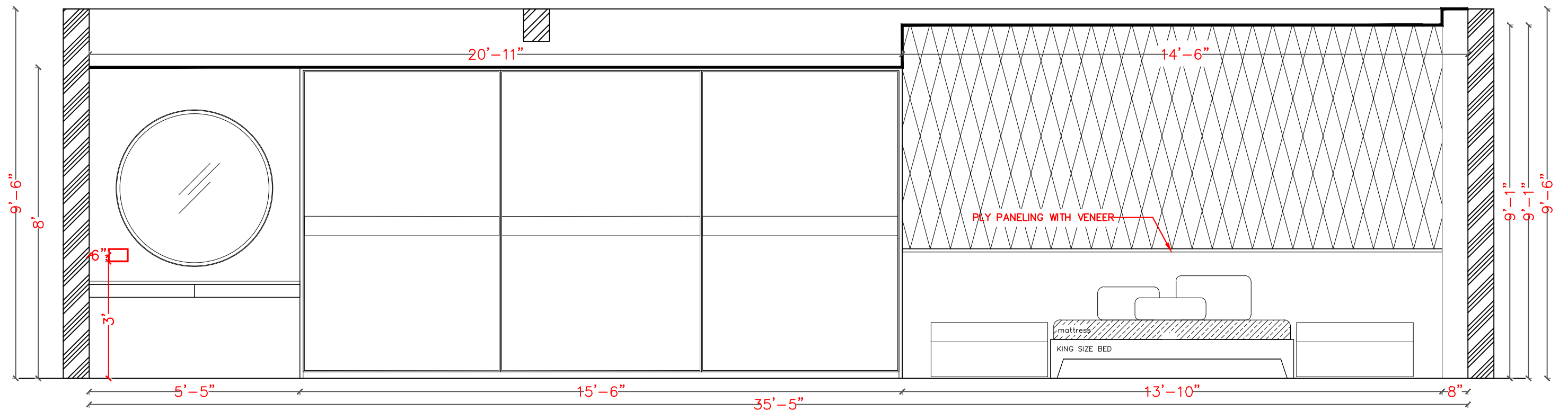
MBR - HEAD WALL ELEVATION
