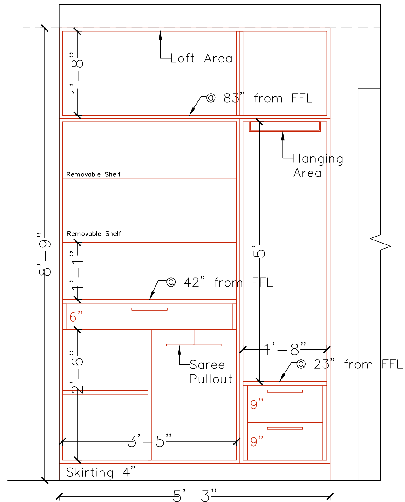
MBR - Bedside Wardrobe Internal Elevation 05.02.2019
