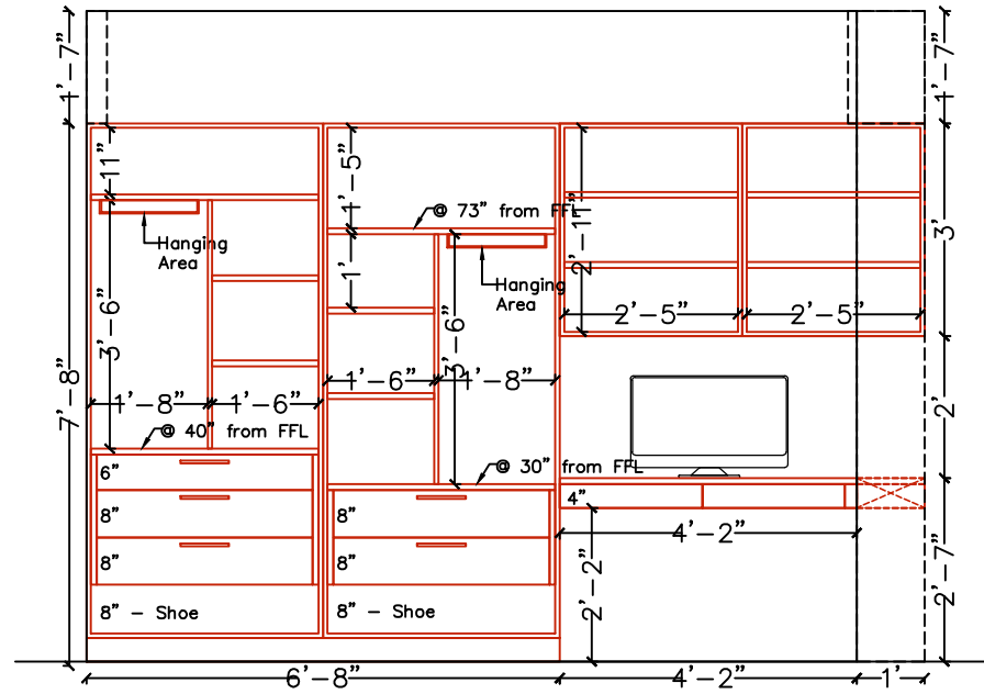
Guest Bedroom – Wardrobe & Study Internal Elevation
