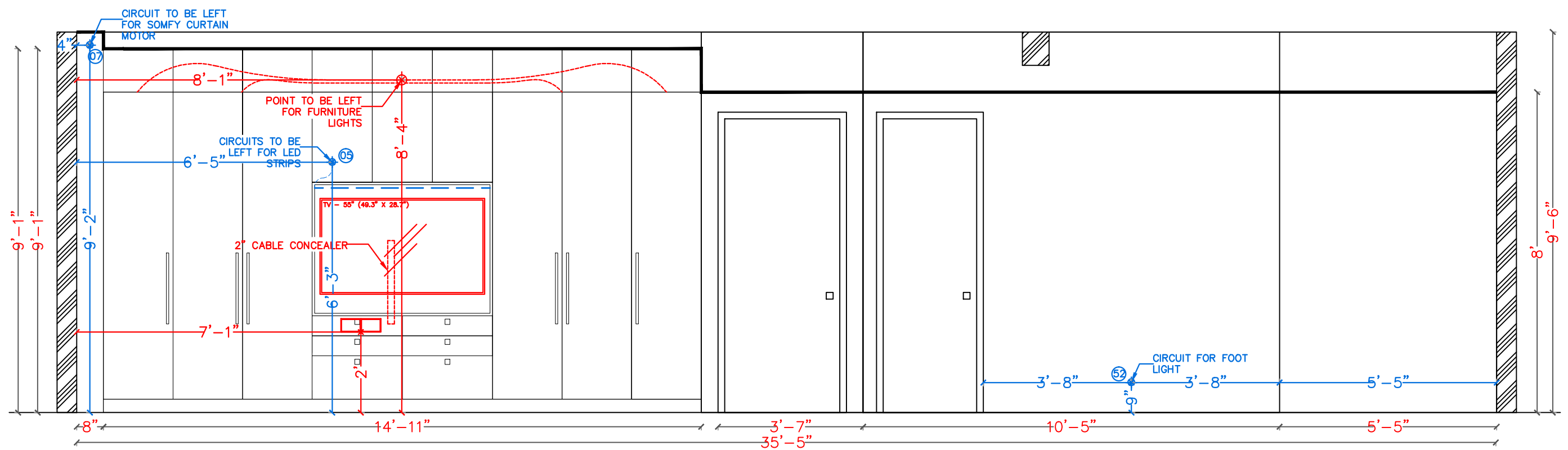
MBR— TV UNIT ELEVATION
