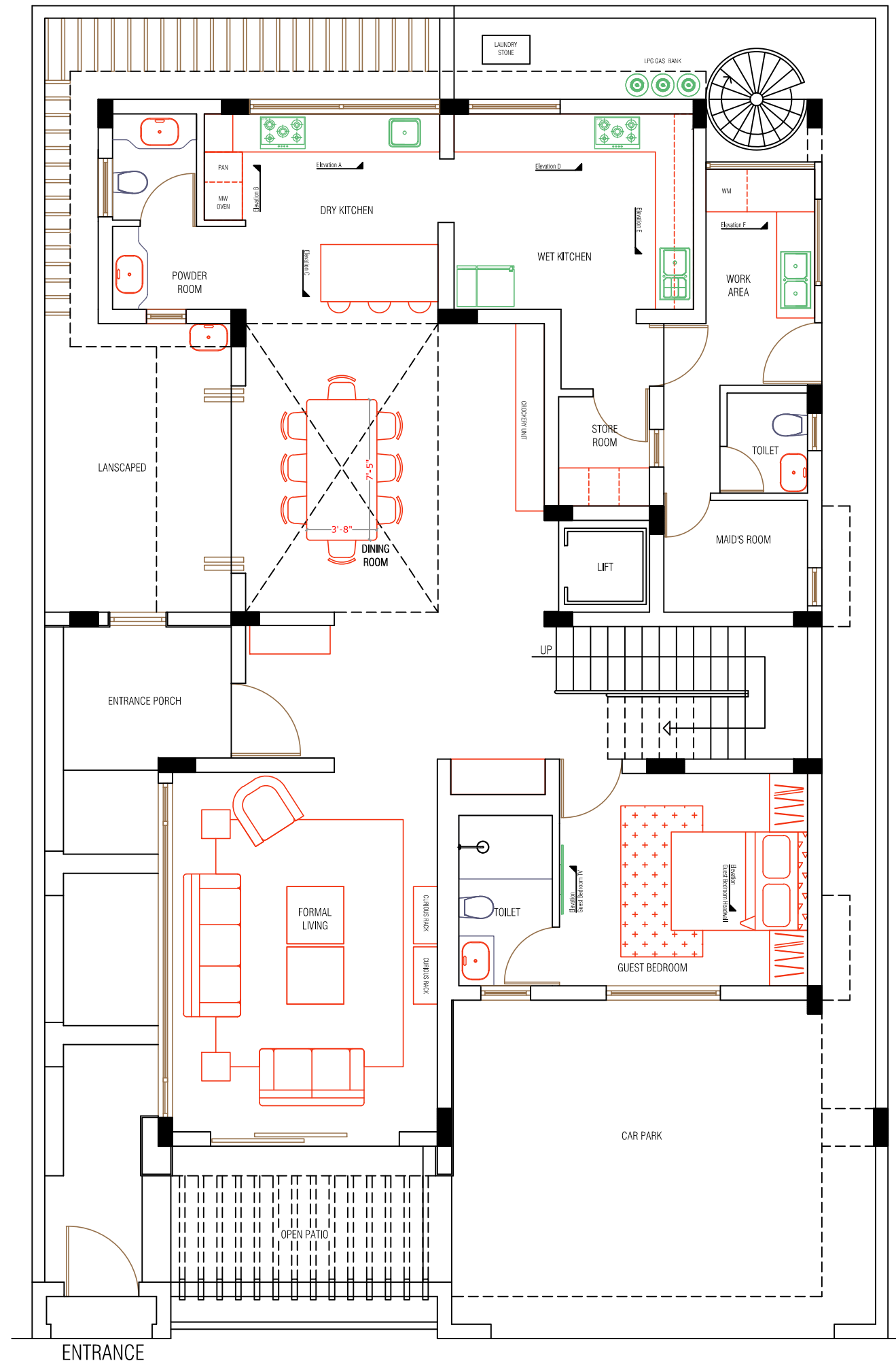
Ground Floor - Furniture Layout - 25.01.2019
