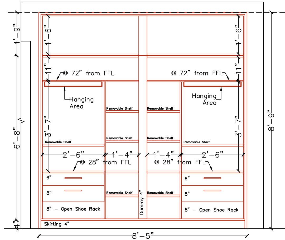
Kids – Sliding Wardrobe Internal Elevation
