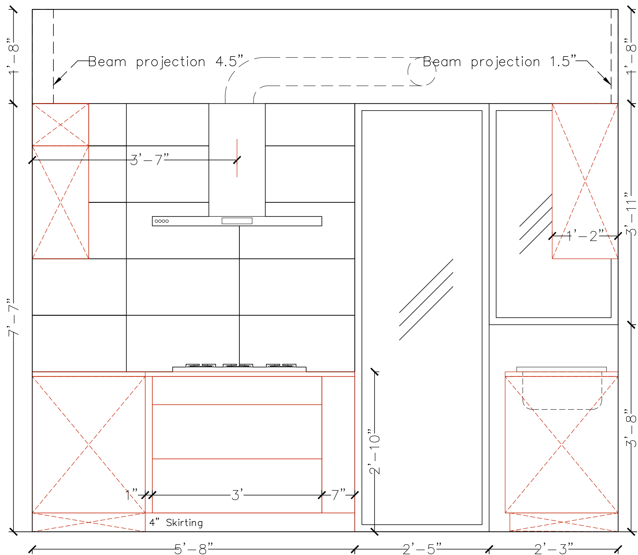
Kitchen — Elevation A
