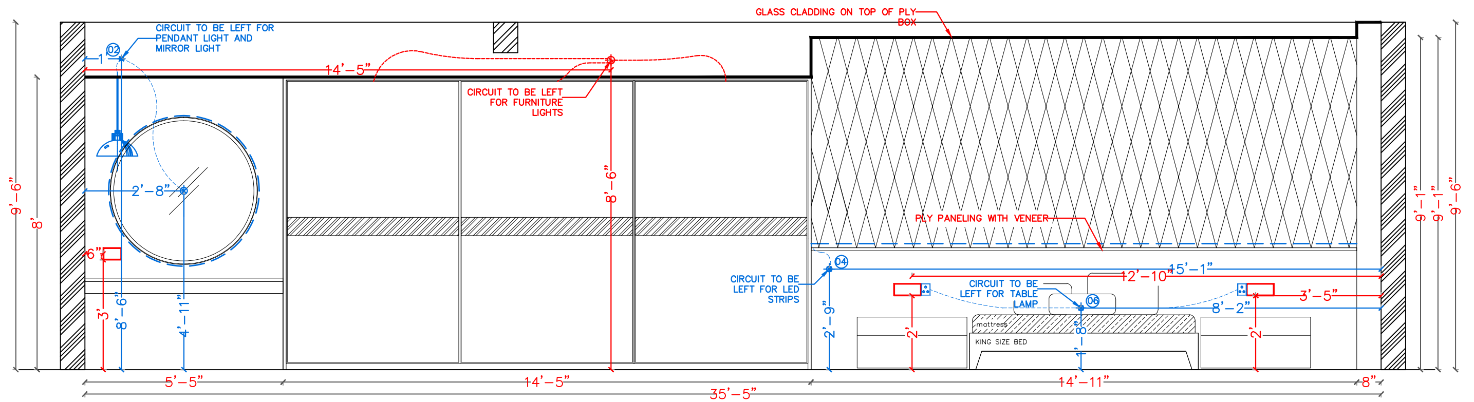
MBR — HEAD WALL ELEVATION
