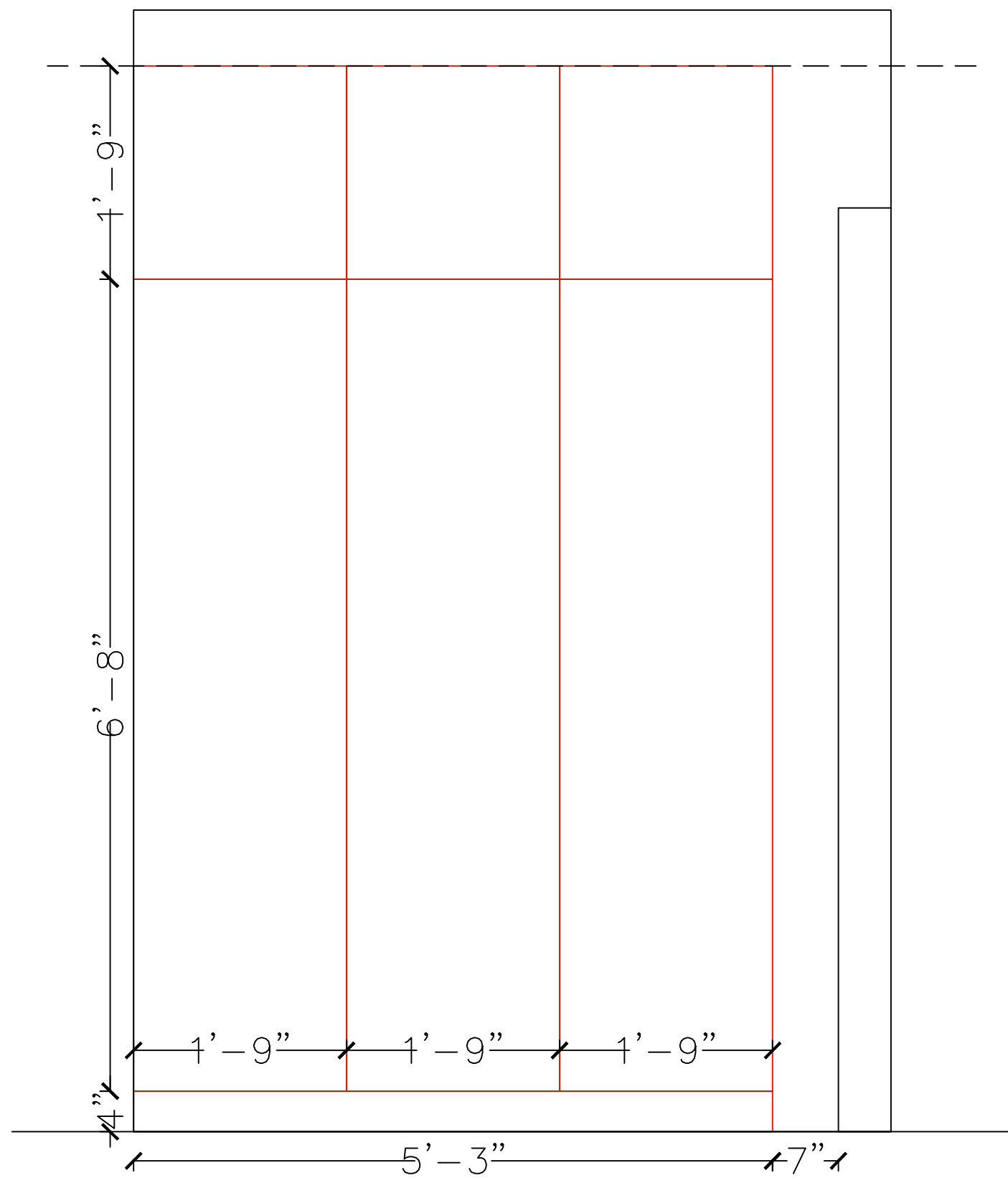
MBR - Bedside Wardrobe - Elevation
