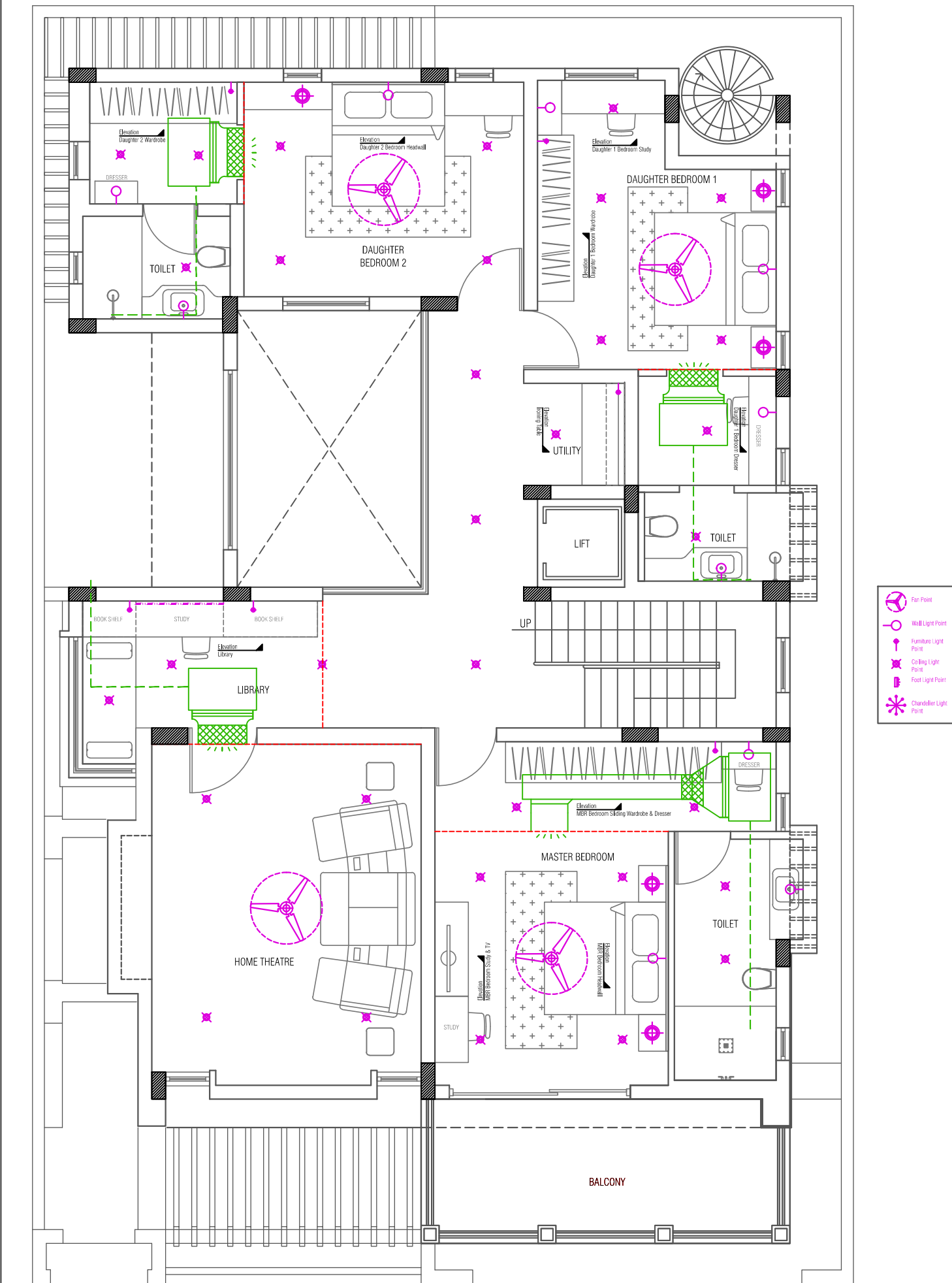
First Floor - Furniture Layout - 07.02.2019
