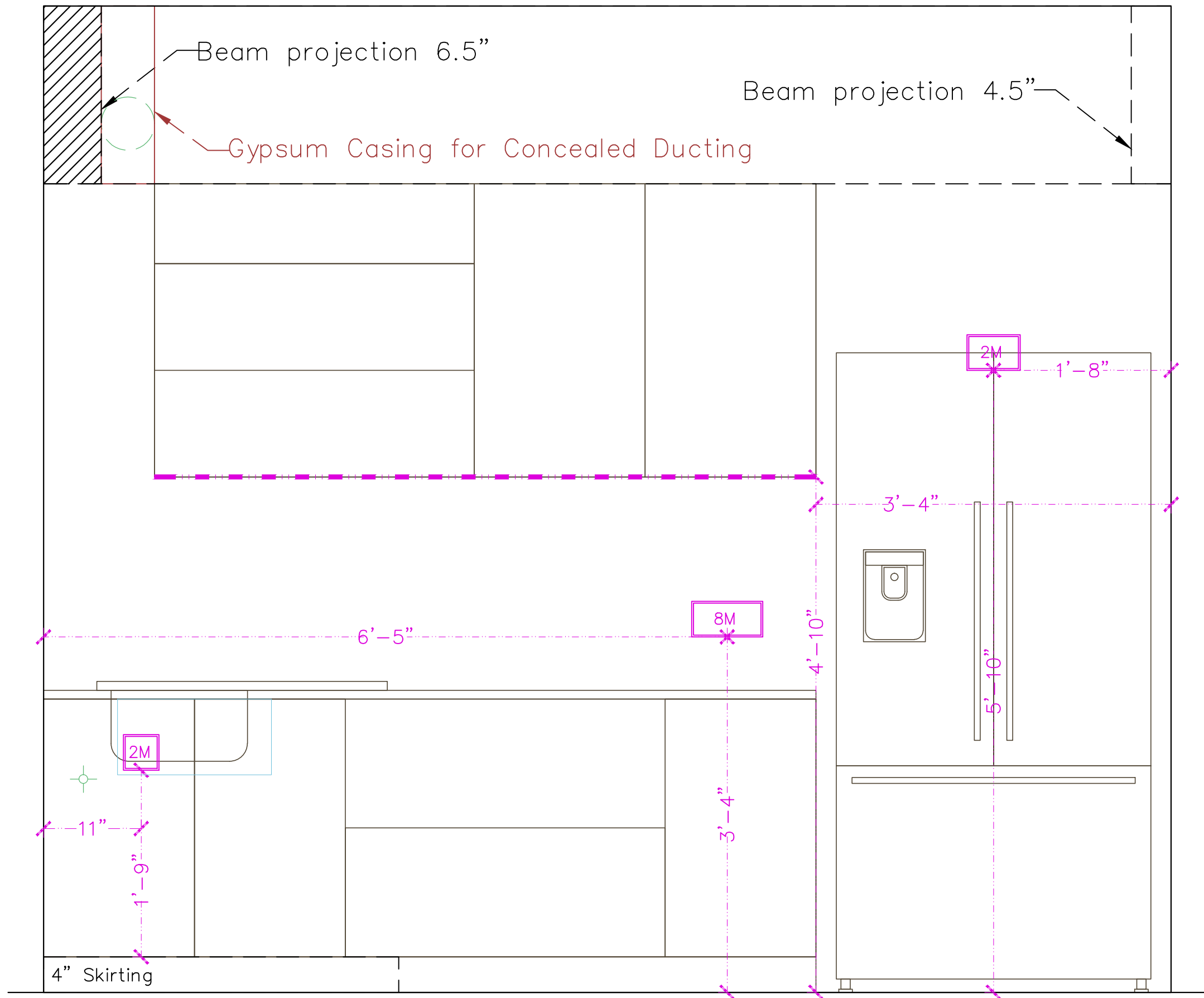
Kitchen — Elevation B
