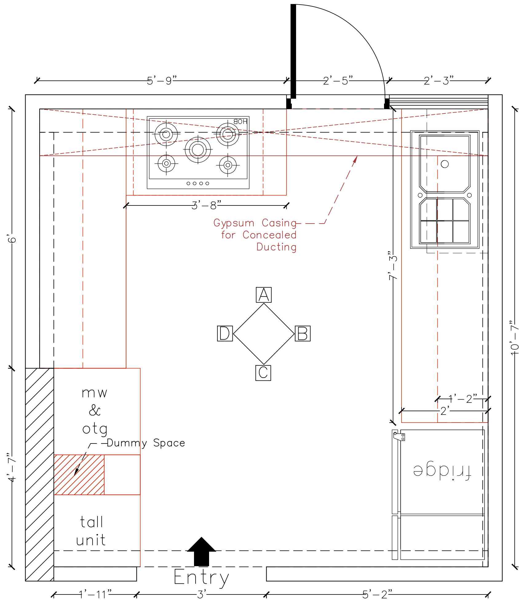
Kitchen – Floor Plan
