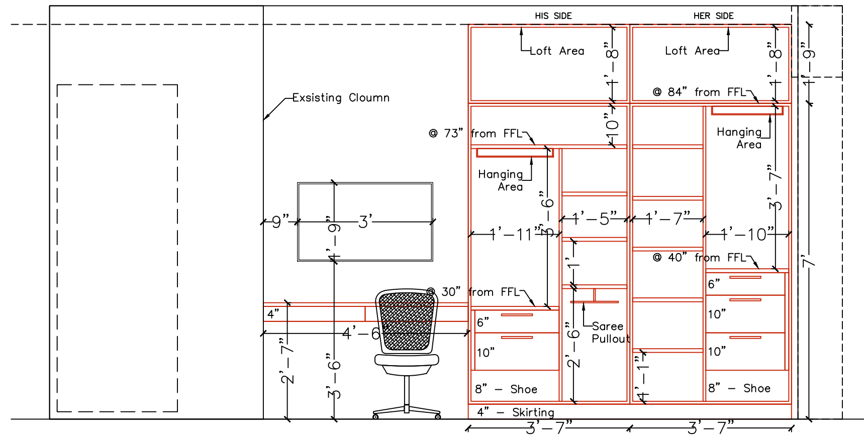
Parents Bedroom – Wardrobe & TV Internal Elevation
