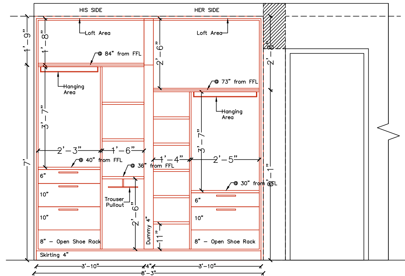
MBR - Sliding Wardrobe - Internal Elevation
