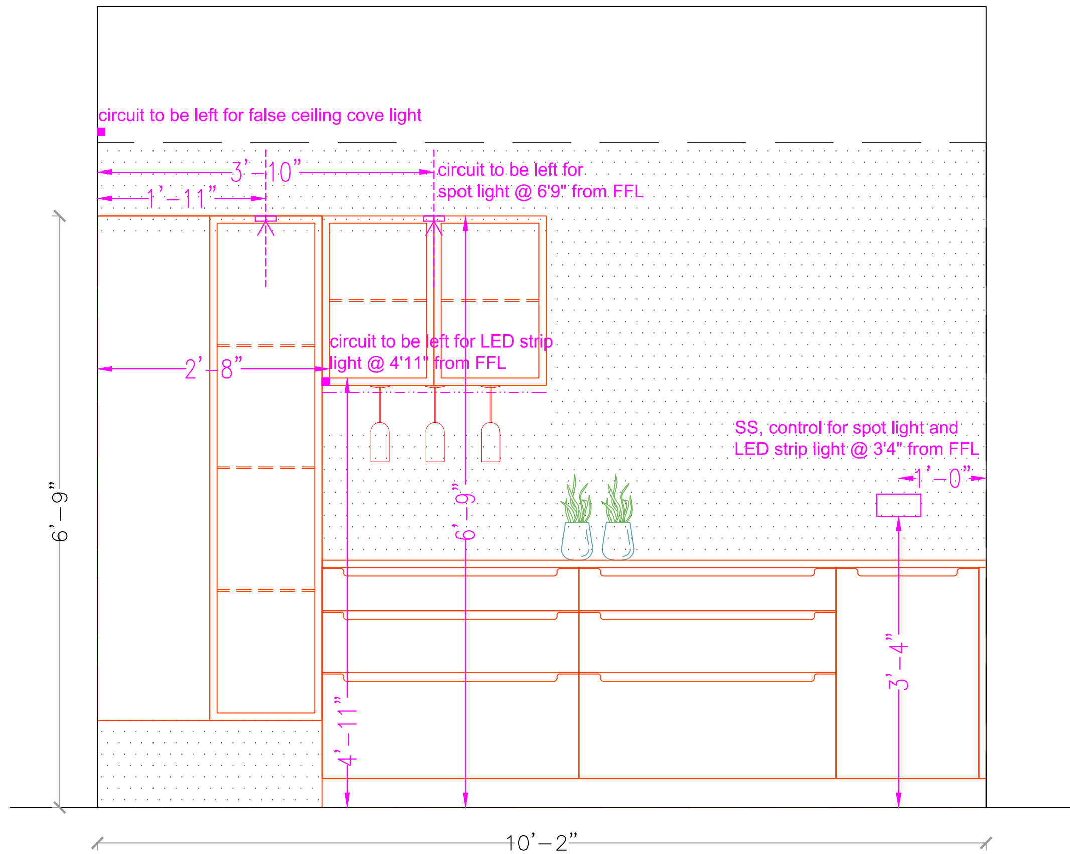
DINING AREA — CROCKERY UNIT — ELEVATION
