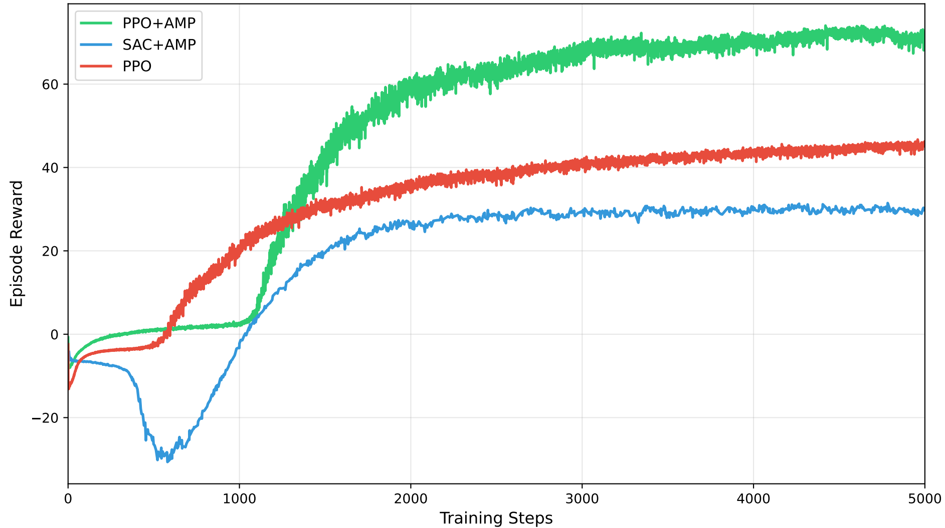
Episode Reward Comparison
