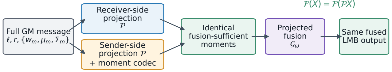
Fig. 1. Receiver-induced message design. The full-message path applies \mathcal{P} at the receiver, whereas the moment-message path applies it before lossless encoding. With matched labels, weights, schedule, delivery masks, and canonical projection—and without quantization or covariance inflation—both paths present identical label-wise moments to \mathcal{G}_\omega and produce the same fused LMB output.
