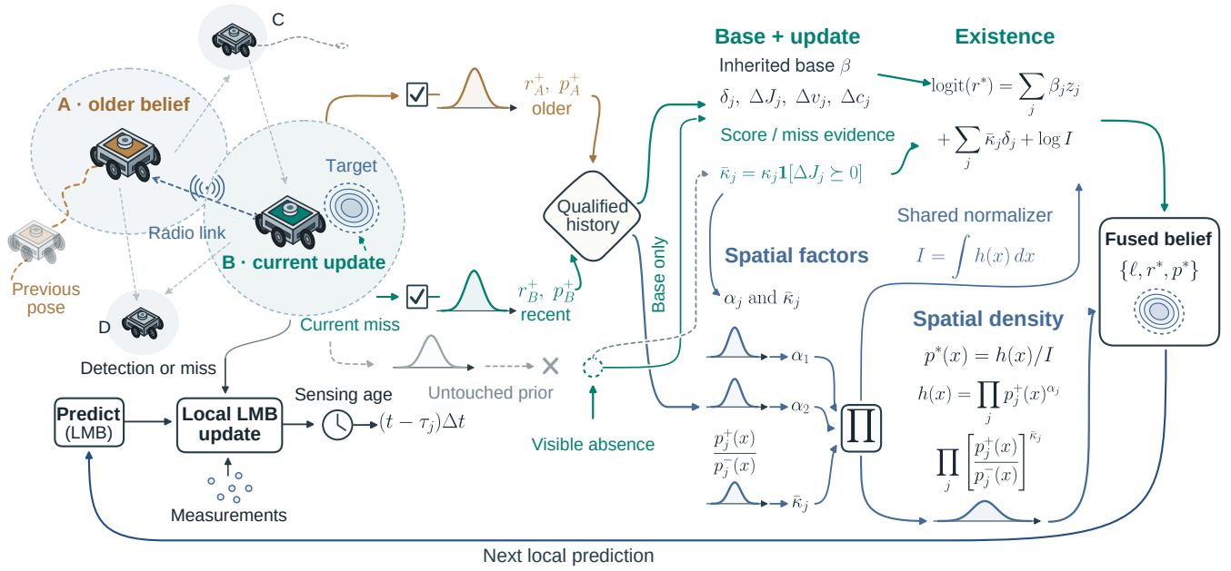
Fig. 2. Guarded current-evidence fusion. Qualified support forms the inherited base. Current correction requires at least two represented sources and no eligible censor; a censor sets every \bar{\kappa}_j = 0 . Sensing, score, and curvature determine admission. The shared integral I couples corrected spatial density and existence. The fused belief becomes the next local prior. Poses and density shapes are illustrative.
