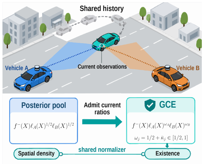
Fig. 1. Cooperative tracking with a common prior, exact local updates, and \alpha_j = \beta_j = 1/2 for j = A, B (illustration). The unnormalized pool f^-(X)\ell_A(X)^{1/2}\ell_B(X)^{1/2} becomes f^-(X)\ell_A(X)^{\omega_A}\ell_B(X)^{\omega_B} under GCE, with \omega_j = 1/2 + \kappa_j \in [1/2, 1] . Joint normalization couples spatial density and existence.
