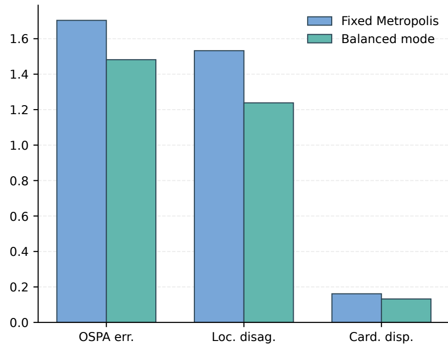
Network Disagreement
