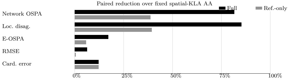
Fig. 3. Paired percentage reductions over the fixed spatial-KLA AA baseline, reported under the validation label Tuned spatial-KLA AA. Black bars show the full label-barycenter operator, and gray bars show the reference-only ablation. The reference-only ablation captures the effect of choosing and copying a consistent local reference label set. The full method gives substantially larger localization and RMSE gains because it also averages matched posterior states.
