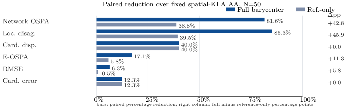
Fig. 2. Mechanism separation in paired percentage reductions. Values are the paired reductions in Table IV relative to the fixed spatial-KLA AA baseline. Blue bars show the full label-barycenter operator, and gray-blue bars show the reference-only ablation. The cardinality rows are shared reference-cardinality controls, not moment-barycenter effects. Spatial E-OSPA/RMSE separation appears only after matched posterior barycenters are added.
