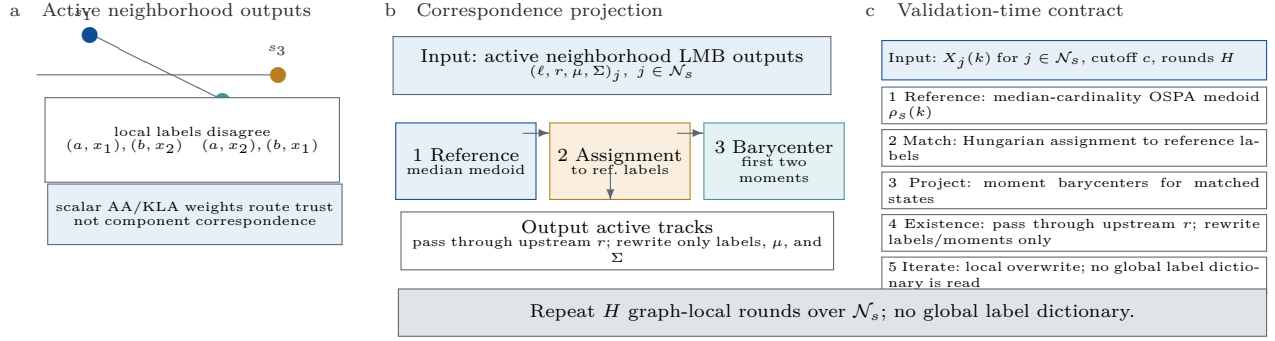
Fig. 1. Active-output correspondence projection. The composite panel shows why scalar fusion weights specify neighbor probability mass but not component correspondence, then gives the graph-local reference, assignment, and moment-barycenter projection used in validation. The input is the active neighborhood LMB output, not a global label dictionary. The operator consumes only graph-neighborhood outputs, passes upstream active-track existence scores through, and rewrites only labels and Gaussian moments.
