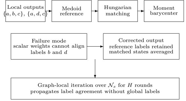
Fig. 1. Core mechanism of the proposed operator. The failure is not only a poor fusion weight: neighboring LMB filters may carry different labels for the same target. The operator first chooses a graph-local reference, then matches neighbor tracks to that reference, and finally averages matched posterior moments.
