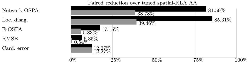
Fig. 3. Paired percentage reductions over the tuned spatial-KLA AA baseline. Black bars show the full label-barycenter operator, and gray bars show the reference-only ablation. The reference-only ablation captures the effect of choosing and copying a consistent local reference label set. The full method gives substantially larger localization and RMSE gains because it also averages matched posterior states.
