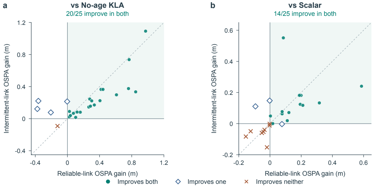
Fig. 2. Sequence-level OSPA gains over (a) No-age KLA and (b) Scalar. Each point pairs the same complete sequence under reliable and intermittent links (25 per panel). Gain is reference minus GCE; the shaded quadrant indicates improvement in both conditions. The dashed diagonal marks equal gains; panel ranges differ.
