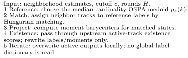
Fig. 2. Validation-time implementation outline. The operator is an estimate-level projection layer: it consumes only graph-neighborhood outputs, does not read a global label set, and does not re-estimate Bernoulli existence probabilities.
