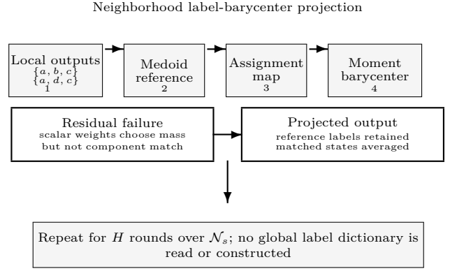
Fig. 1. Core mechanism of the proposed operator. Fusion weights specify how much probability mass a neighbor contributes, but they do not define component correspondence across local LMB posteriors. The operator therefore chooses a graph-local reference, matches neighbor tracks to that reference, and replaces matched states by posterior moment barycenters.
