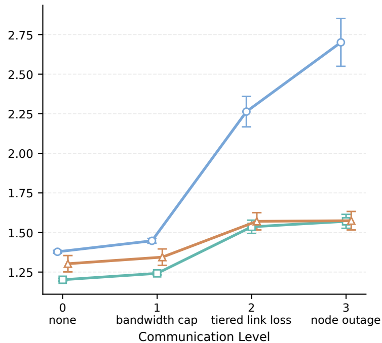
Matched Localization Disagreement
