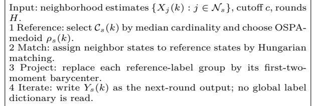
Fig. 2. Implementation outline used in the validation. The operator is an estimate-level projection layer: it consumes only graph-neighborhood outputs and does not read a global label set.
