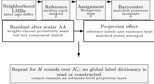
Neighborhood label-barycenter projection graph-local label alignment before moment fusion
