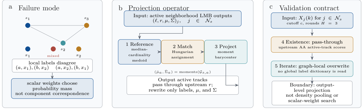
Fig. 1. Active-output correspondence projection. Scalar weights route probability mass but do not infer component correspondence. The operator chooses a graph-local reference, assigns neighbor tracks to it, and moment-matches the assigned states. Existence scores pass through from upstream AA; only labels and Gaussian moments are rewritten, with no global label dictionary.
