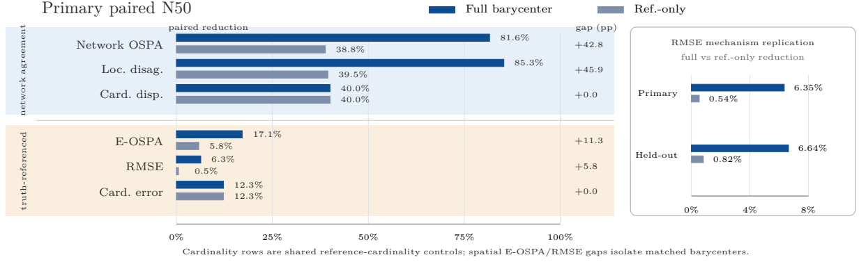
Fig. 2. Mechanism separation in paired percentage reductions. Blue bars show the full label-barycenter operator, gray-blue bars show the reference-only ablation, and the right inset repeats the RMSE separation for the primary and held-out N50 runs. Cardinality rows are shared controls; the spatial E-OSPA/RMSE gap appears only after matched posterior barycenters are added.
