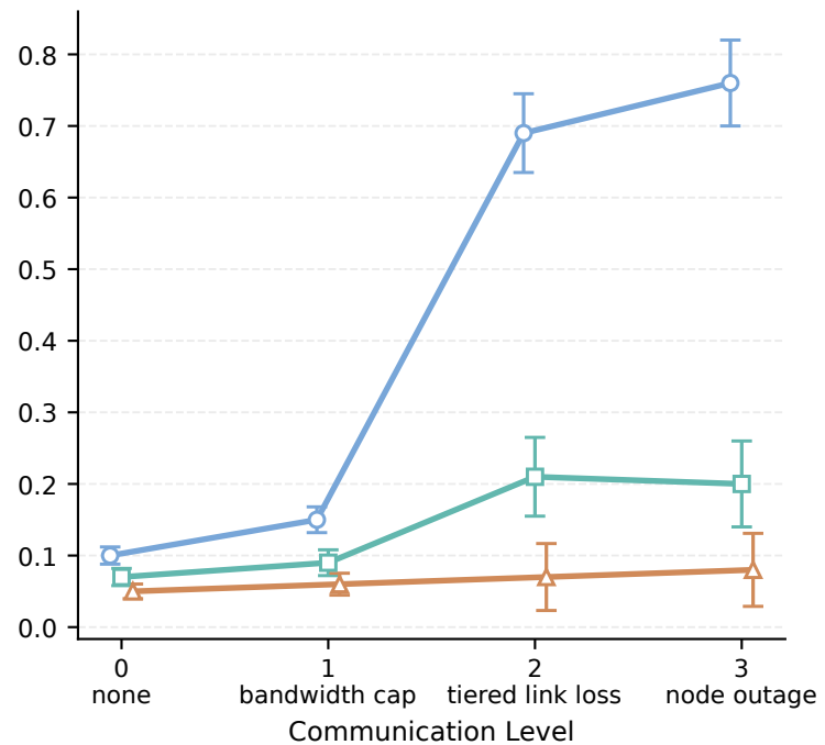
Cardinality Dispersion
