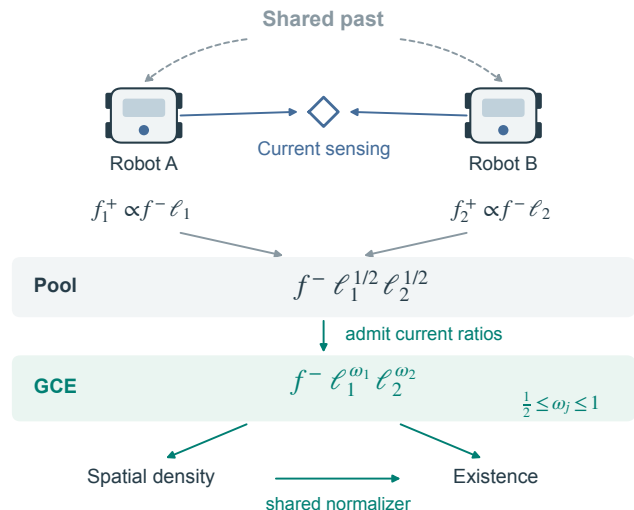
Fig. 1. Separating current sensing from inherited information. In the idealized two-robot shared-prior case, geometric pooling retains the prior but tempers each current likelihood. GCE admits bounded fractions of current posterior-to-prediction ratios, increasing the likelihood exponents \omega_j while retaining one prior. Joint normalization carries this correction into both spatial density and existence.
