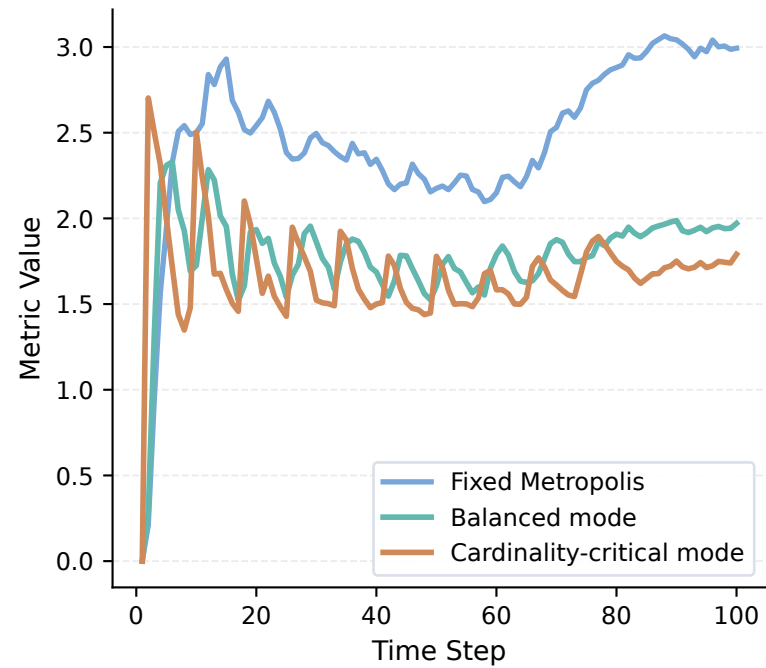
OSPA consensus error
