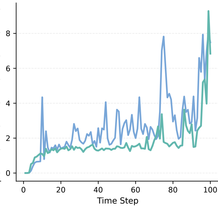
Consensus RMSE
