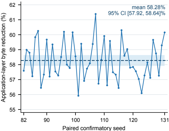
a Per-seed communication reduction
