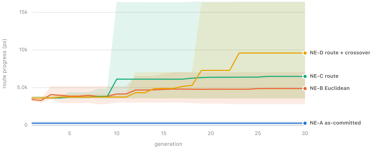
Fig. 9. Learning curves: best route progress reached by the champion of each generation, averaged over seeds, with the band spanning the minimum and maximum across seeds. The as-committed arm is flat by construction.
