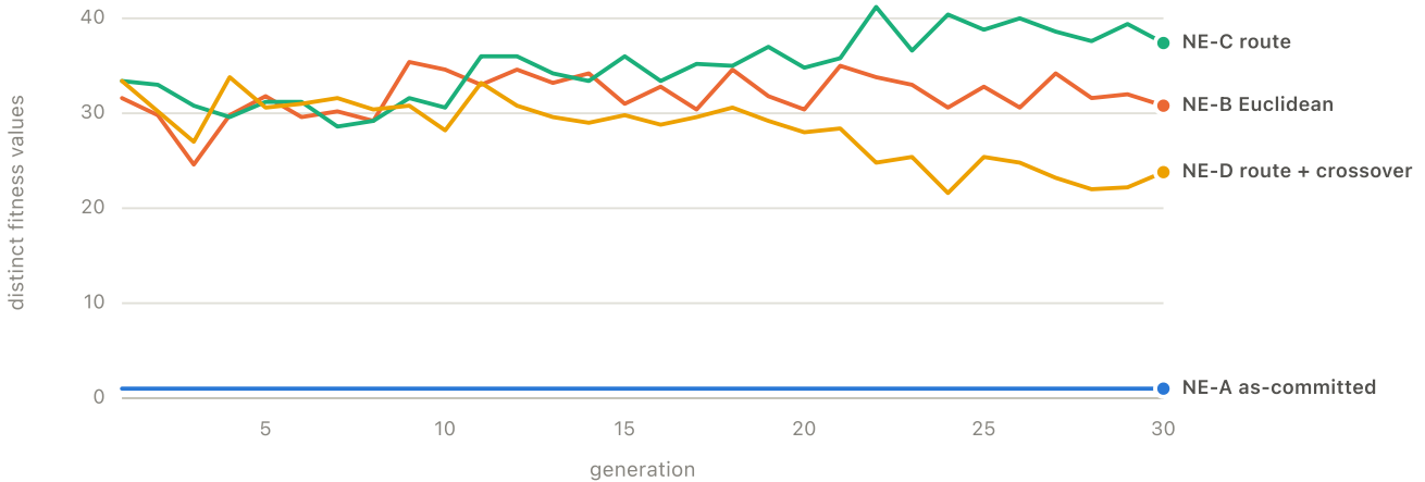
Fig. 10. Distinct fitness values per generation. This is the quantity that determines whether selection can act at all; the as-committed arm sits at exactly one for the entire run, in every seed.
