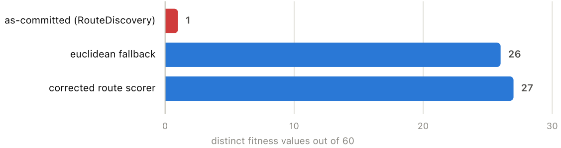
Fig. 7. Selection signal available to the genetic algorithm. The as-committed objective yields a single distinct fitness value across the whole population, so the champion is chosen arbitrarily.
