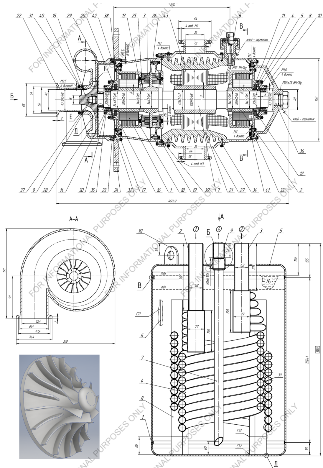
Figure 1: Designed apparatus
