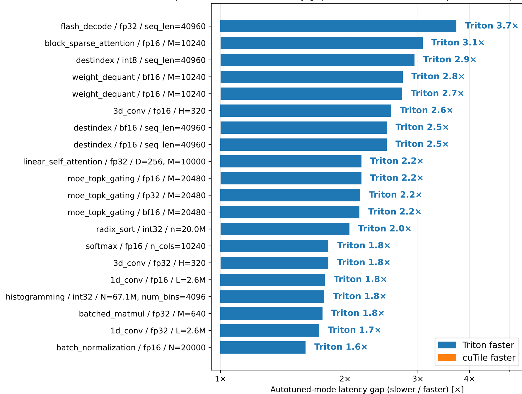
Top 20 Triton vs cuTile latency gaps (autotuned mode, NCU-profiled sweep-max input)
