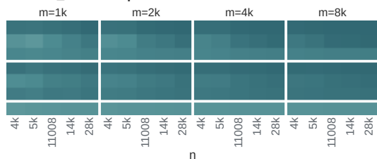
streamk_matmul · fp32
