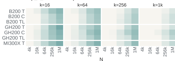
top_k_selection · fp32
