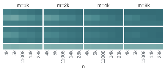
streamk_matmul · bf16
