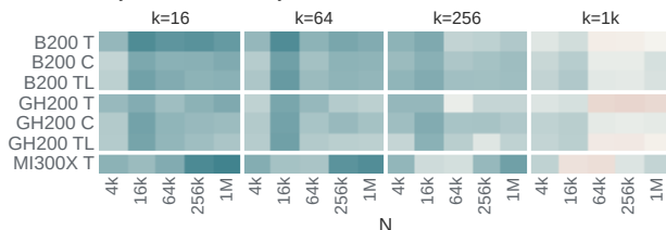
top_k_selection · fp32
