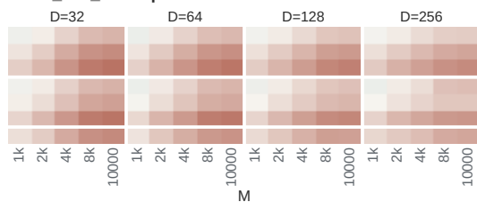
streamk_matmul · bf16
