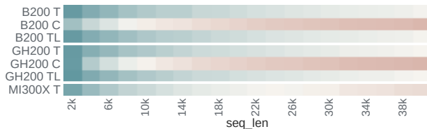
top_k_selection · fp32
