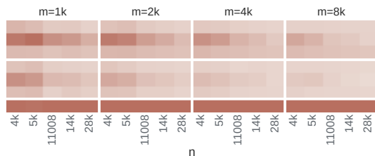
streamk_matmul · fp32
