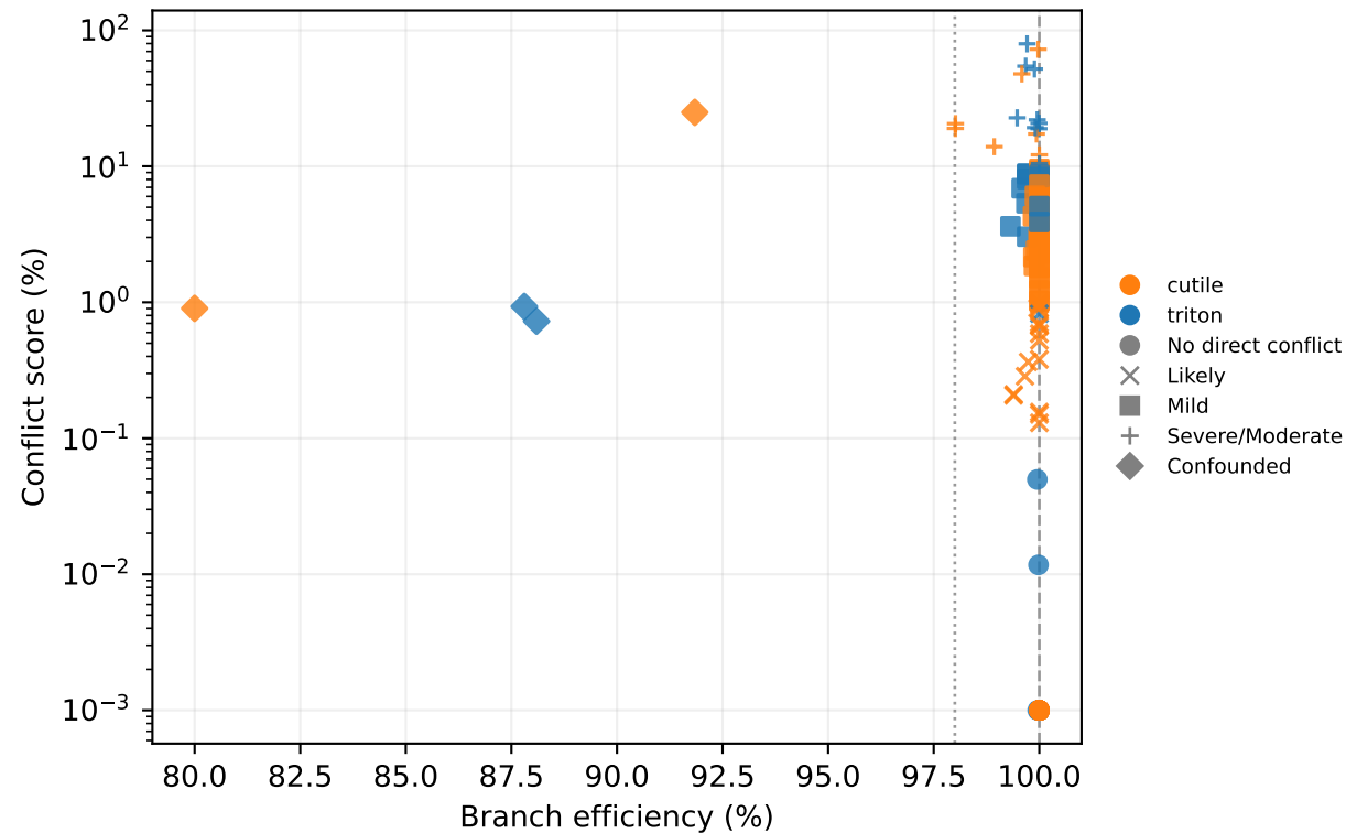
Branch-divergence confounder
