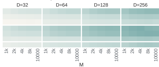
streamk_matmul · bf16
