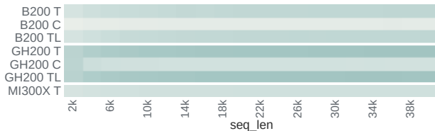
top_k_selection · fp32
