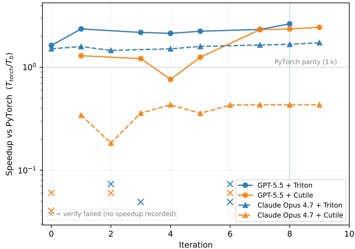
Iterative convergence: softmax
