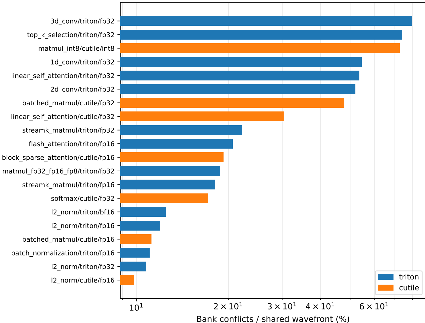
Top 20 bank-conflict cases
