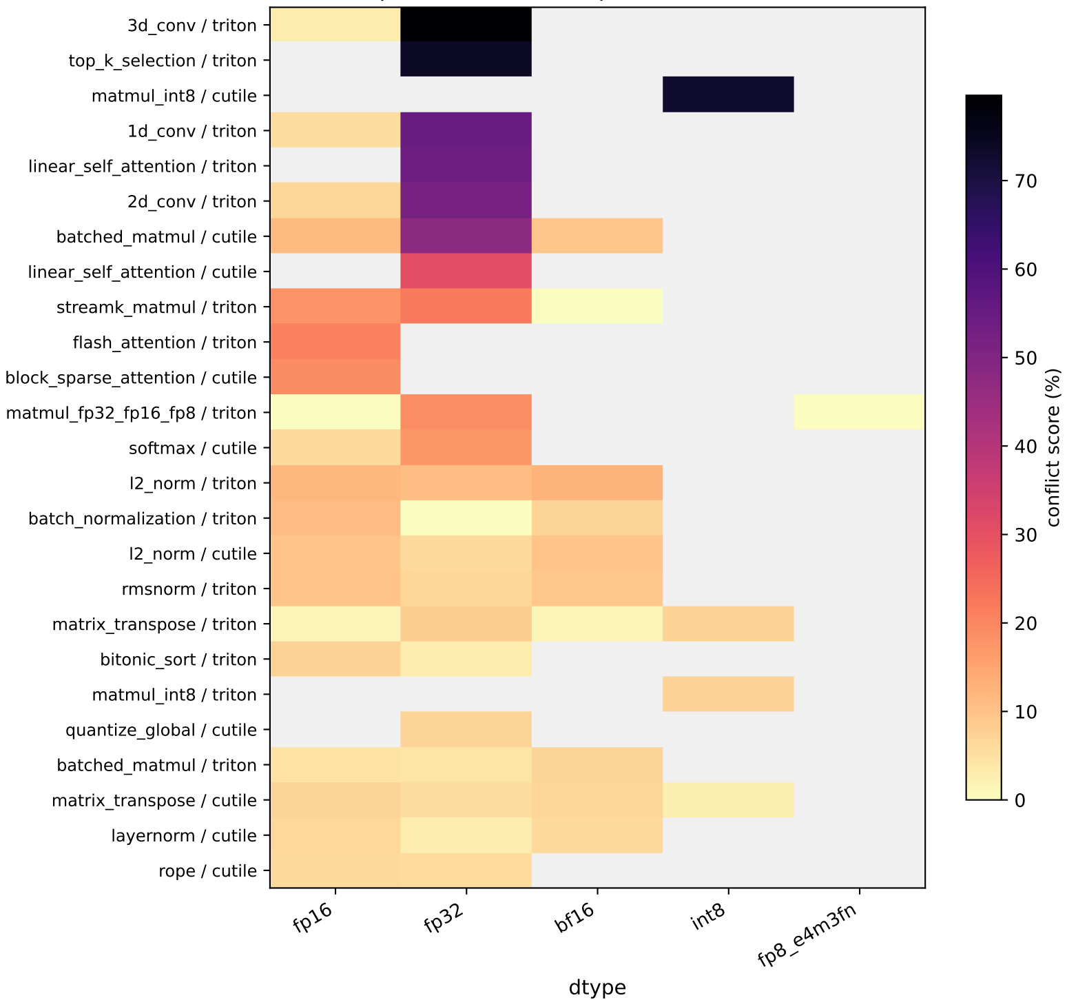
Top 25 bank-conflict operator/backend rows
