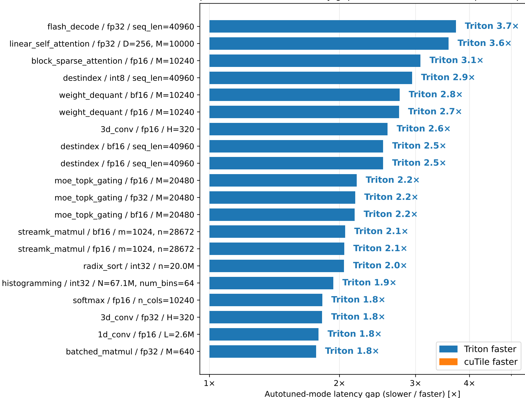
Top 20 Triton vs cuTile latency gaps (autotuned mode, sweep-max input)
