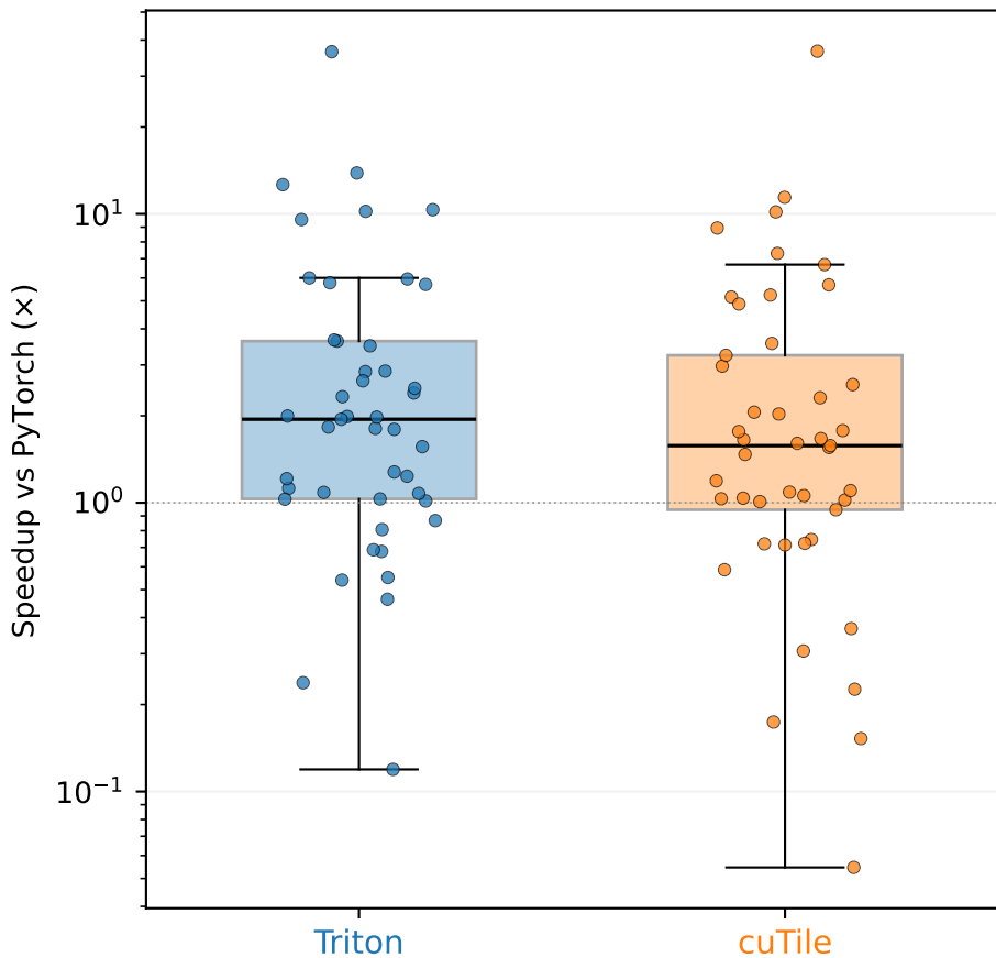
Autotuned mode (vs PyTorch)
