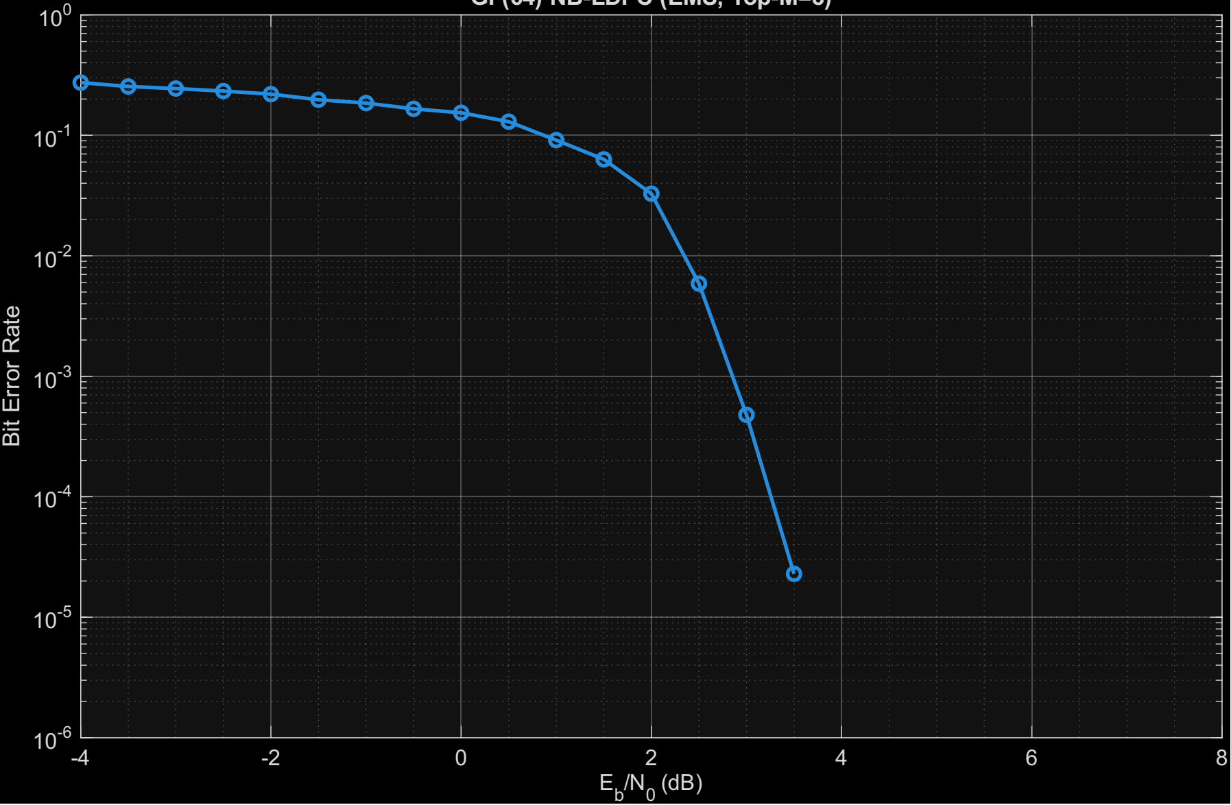
GF(64) NB-LDPC (EMS, Top-M=8)
