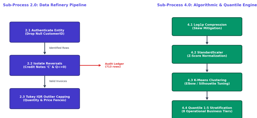
Figure 2.3: Level 2 Data Flow Diagram (Refinery & ML Decomposition)
