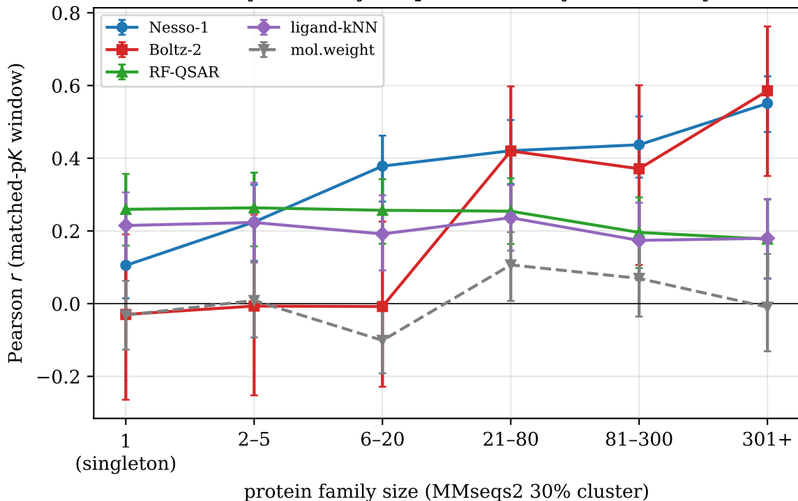
Affinity accuracy vs. protein-family redundancy
