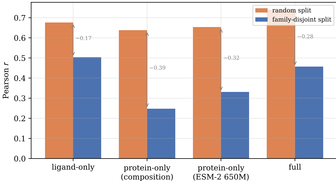
Random-split accuracy is protein-family memorization
